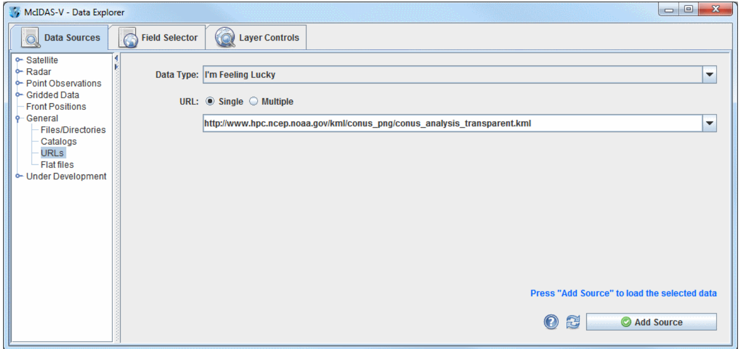
Image 1: URL Chooser
