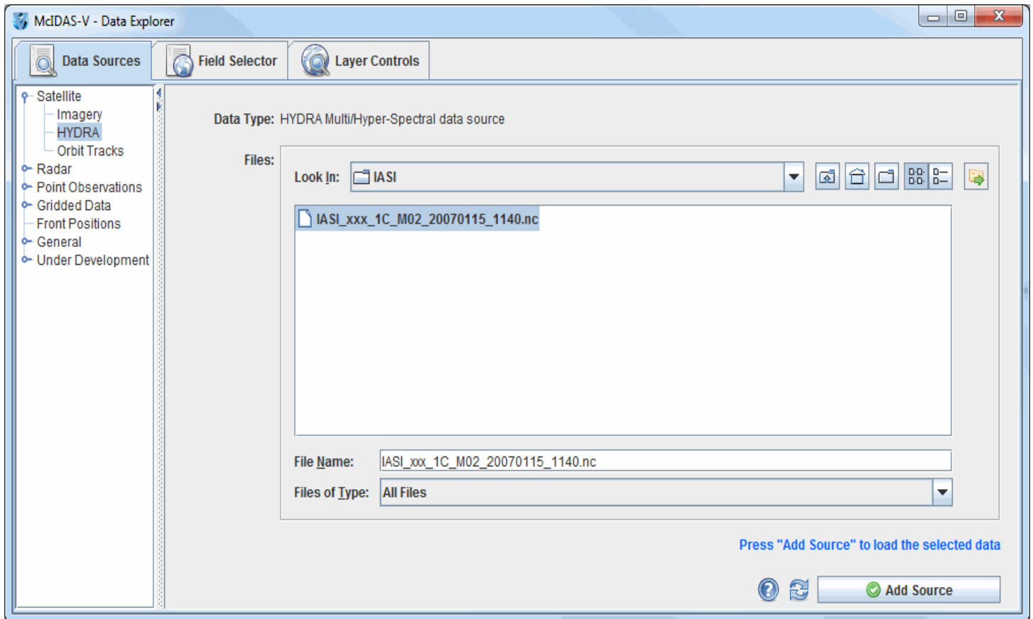
Image 1: HYDRA Chooser
