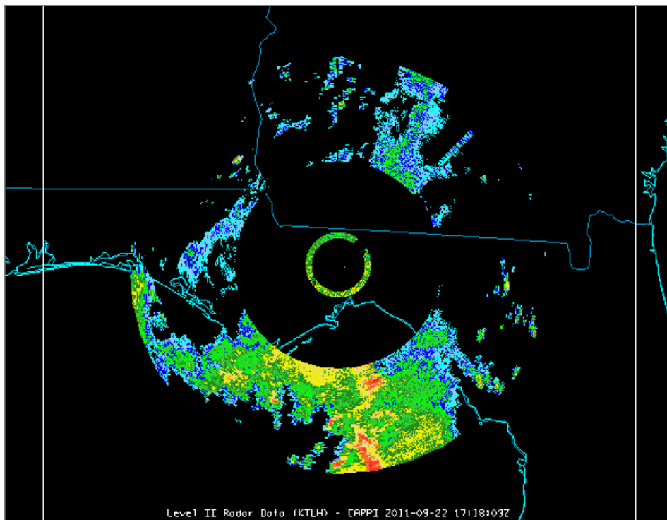
Image 7: CAPPI Display
