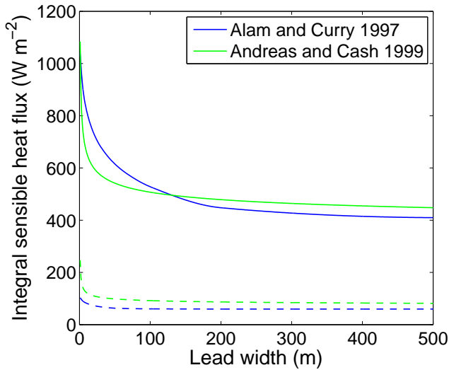
Fig. 2. Integral sensible heat flux as function of lead width computed using the methods of Alam and Curry (1997) – blue – and of Andreas and Cash (1999) – green. Solid and dashed lines correspond to \Delta T = 30^\circ\text{C} , U = 7\text{ m s}^{-1} and \Delta T = 10^\circ\text{C} , U = 3\text{ m s}^{-1} , respectively.
