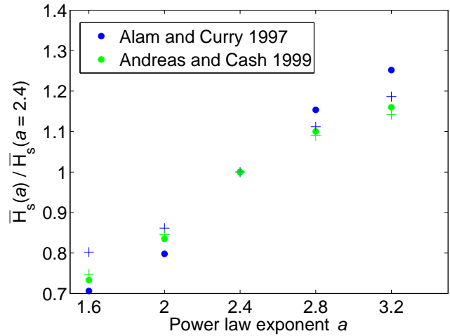
Fig. 6. Ratios of the sensible heat fluxes calculated using the methods of Andreas and Cash (1999) – green – and of Alam and Curry (1997) – blue – for several distributions of lead width exponents a to the fluxes calculated for a = 2.4 , as a function of a for two atmospheric conditions: \Delta T = 30^\circ\text{C} , U = 7 \text{ m s}^{-1} (dots) and \Delta T = 10^\circ\text{C} , U = 5 \text{ m s}^{-1} (plus).
