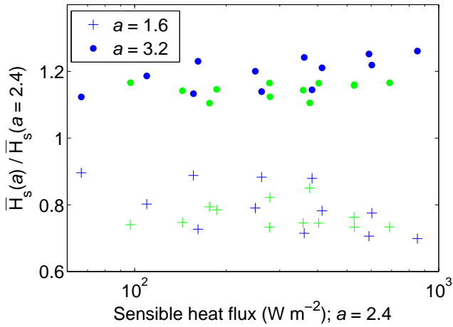
Fig. 5. Ratios of the sensible heat fluxes calculated using the methods of Andreas and Cash (1999) – green – and of Alam and Curry (1997) – blue – for two distributions of lead width exponents: a = 1.6 (plus) and a = 3.2 (dots) to the fluxes calculated for a = 2.4 , for the same atmospheric conditions as in Table 1.
