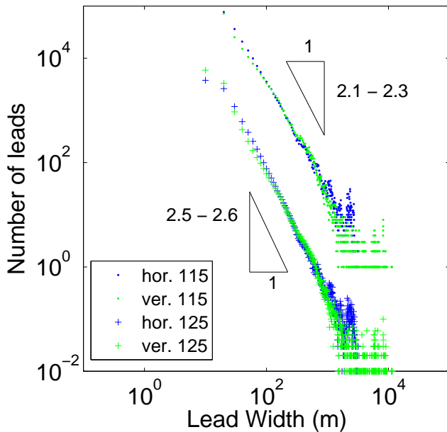
Fig. 4. Lead-width distribution along all vertical or horizontal transects on the SPOT image for the two different thresholds. We have divided the distribution associated to th=125 by a factor 100 for clarity purposes. The triangles are here to indicate the slope of the plots.
