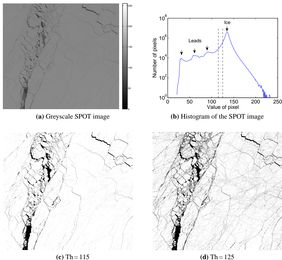
Fig. 3. (a) Greyscale satellite SPOT image of the sea ice cover of size 5977 \times 6618 pixels taken 6 April 1996 (i.e. early spring), centered around 80^\circ 11' N , 108^\circ 33' W covering 60 \times 66 \text{ km}^2 . On the right is the luminance scale of the picture. (b) Pixel color histogram of the SPOT image; the dashed lines correspond to the two thresholds 115 and 125. (c) and (d) Binary images for th = 115 and th = 125 .
