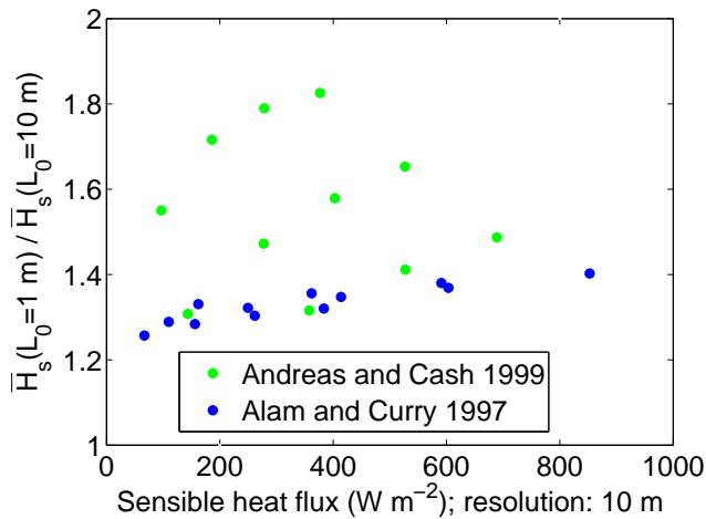
Fig. 7. Ratio of the sensible heat fluxes calculated with resolution L_0 = 1 m to L_0 = 10 m using the methods of Andreas and Cash (1999) – green – and of Alam and Curry (1997) – blue – for the same power law exponent a = 2.4 and for the same atmospheric conditions as in Table 1. Note that in this calculation, the four points in the upper left corner are obtained using the method of Andreas and Cash (1999) for low wind speed ( U = 3 \text{ m s}^{-1} ).
