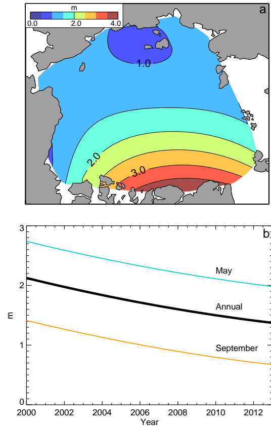
Figure 4. (a) Mean annual ice thickness from the ITRP for the period 2000–2012. (b) Mean ice thickness for the Arctic Basin in May, in September, and for the annual mean.
