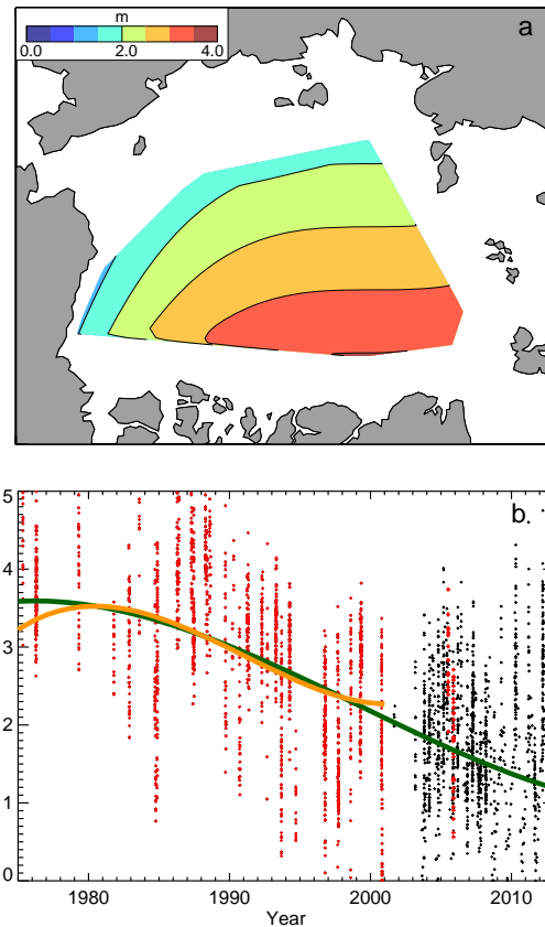
Figure 5. (a) Map of the annual mean ice thickness in the SCICEX box and (b) time series of the annual mean. The orange line is the third-order polynomial from RPW08 for which the draft was converted to thickness with a factor of 1.107. The green line is a third-order polynomial from this study. The dots show the observations from within the box; red are from the submarines.
