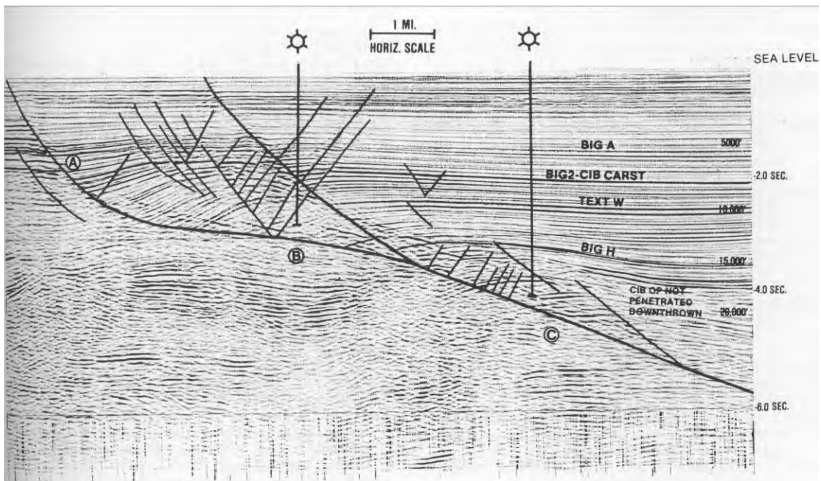
Figure 2-8. An example of a growth fault in the Gulf Coast across Coair fault trend, offshore Texas. This seismic section shows a listric segment of the fault (A), a bedding parallel slide surface that rests on overpressured shale (B), and a deep ramp that changes orientation of the slide surface (from Vogler and Robinson, 1987). Reprinted by permission of the AAPG whose permission is required for further use.
