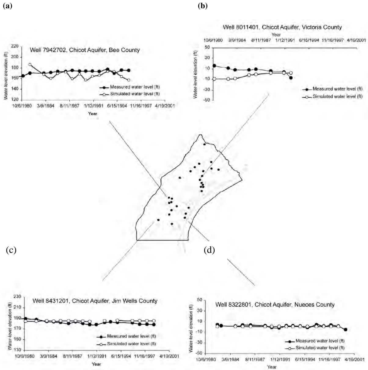
Figure 10-11. Comparison of simulated and measured water-level fluctuations in several wells for 1980 through 1999 for (a) well 7942702, (b) well 8011401, (c) well 8431201, and (d) well 8322801 for the GAM of the central part of the Gulf Coast aquifer (from Chowdhury and others, 2004).
