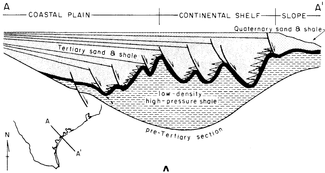
Figure 2-7. Diagrammatic crosssection along the central part of the Texas Gulf Coast and northern Gulf of Mexico basin showing depositional and structural styles exhibited by fluvial deltas (from Bruce, 1973 and Solis, 1981).
