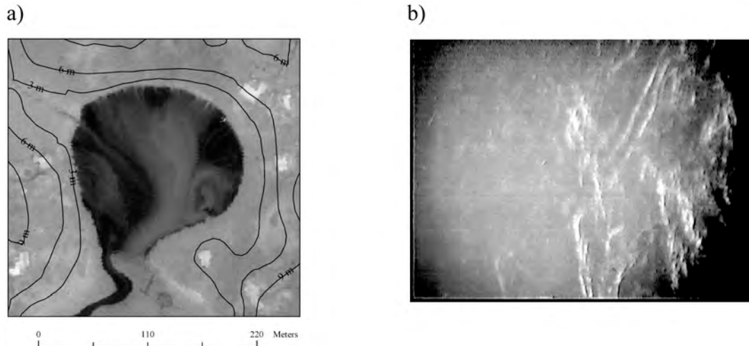
Figure 9-1. Though in many ways difficult to observe, submarine groundwater discharge can be imaged by a) infrared photography (image provided by Ann Mulligan and Matt Charette) and b) ‘schlieren’ photographic techniques sensitive to the density differences between saline and fresh or brackish groundwater (reprinted from Karpen and others, 2004, copyright 2003, with permission from Elsevier). In this a) thermal infrared aerial photograph of a tidal pond near Waquoit Bay, MA, the cooler (lighter) groundwater discharge can be seen mixing with the warmer (darker) bay water (Mulligan and Charette 2005). In b) a specially designed underwater ‘schlieren’ photographic system images submarine seepage several kilometers offshore in the Baltic Sea (Karpen and others, 2004).
