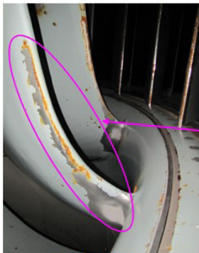
Inlet Suction
