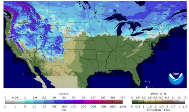
Sample snow depth output from Snow Data Assimilation System for January 15, 2015. Image courtesy of the National Oceanic and Atmospheric Administration.
