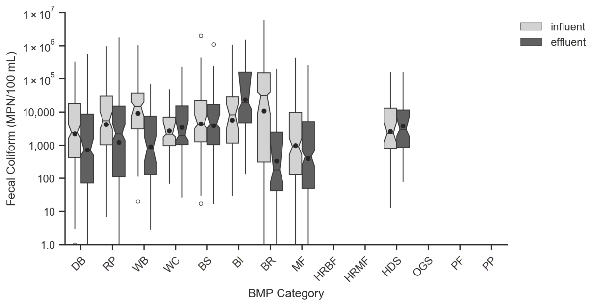
Figure 3-4. Box Plots of Influent/Effluent Fecal Coliform (cfu/100 mL).
