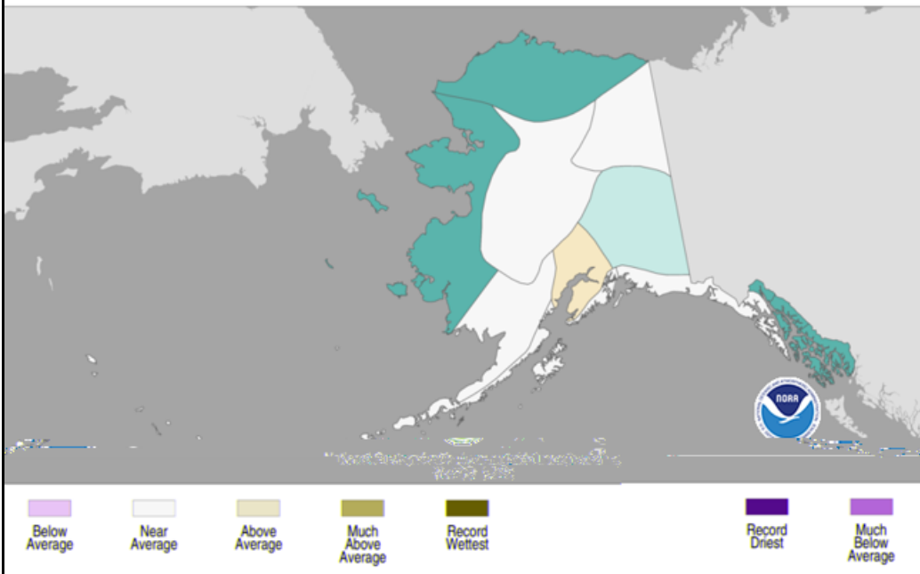
Alaska Divisional Precipitation Ranks October 2020–September 2021 Period: 1925–2021
