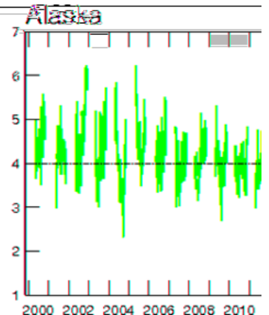
Average Streamflow Percentile and Index at 12 primary USGS Gages in Alaska. Images: USGS (waterwatch.usgs.gov).
