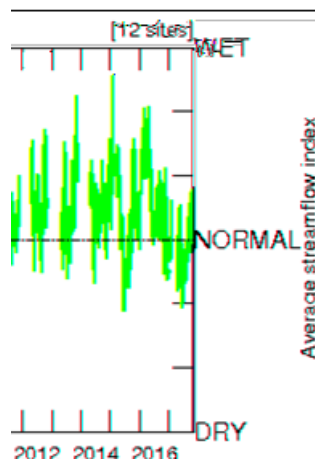
Average Streamflow Percentile and Index at 12 primary USGS Gages in Alaska. Images: USGS (waterwatch.usgs.gov).
