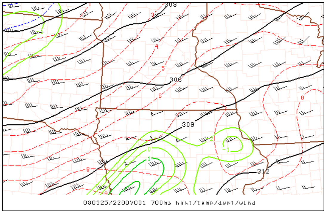
Fig. 3. 700-mb height, temperature, dewpoint, wind 2200 UTC 25 May 2008
