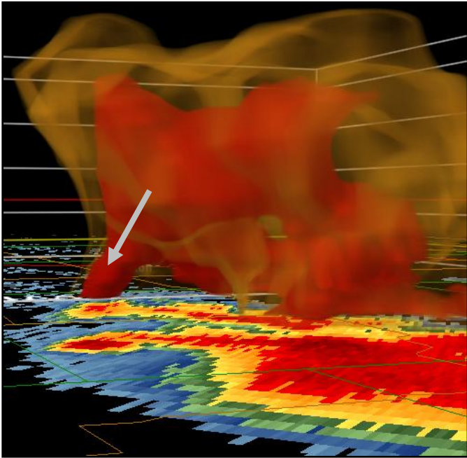
Fig. 21. Volumetric reflectivity, 2208 UTC 25 May 2008
