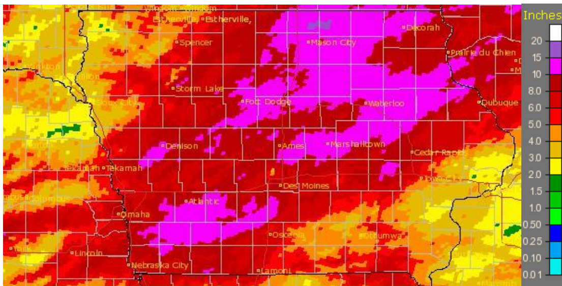
Figure 4: June 12, 2008 radar-estimated total rainfall across Iowa for 14 days ending on the 12 th .
