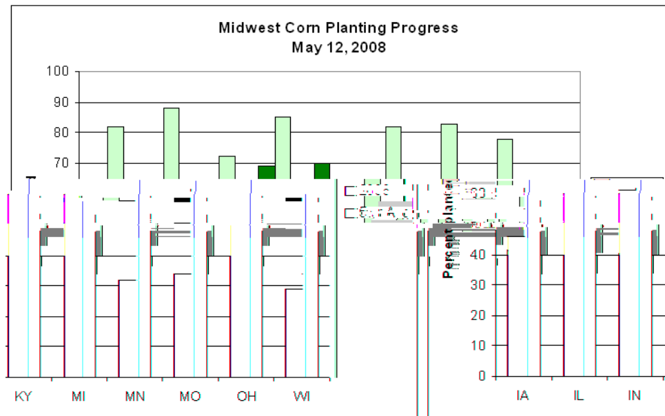
Figure 25: Midwest corn planting progress by mid-May 2008
