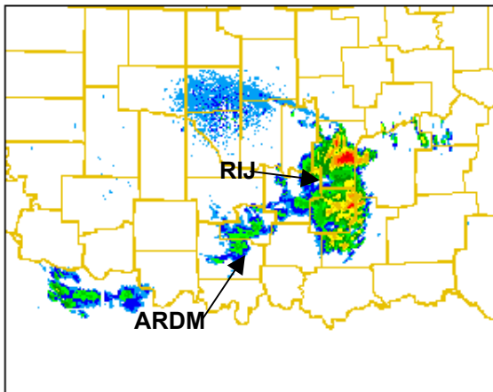
Figure 2. Base reflectivity image at the 0.5 degree elevation slice from the Twin Lakes (KTLX) WSR-88D at 0826 UTC, on 15 May 1995.
