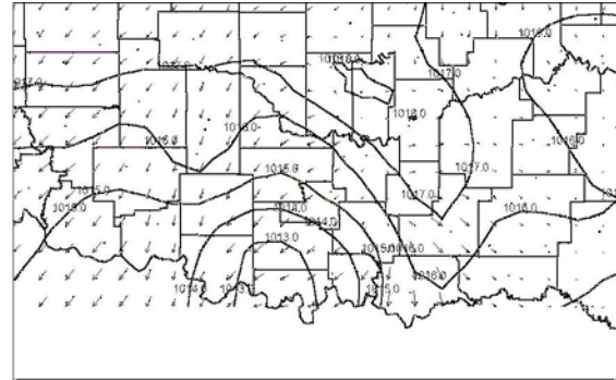
Figure 3. Analysis of sea level pressure and surface wind vectors from the Oklahoma Mesonet at 0825 UTC on 15 May 1995. Pressure is analyzed every 1 mb.
