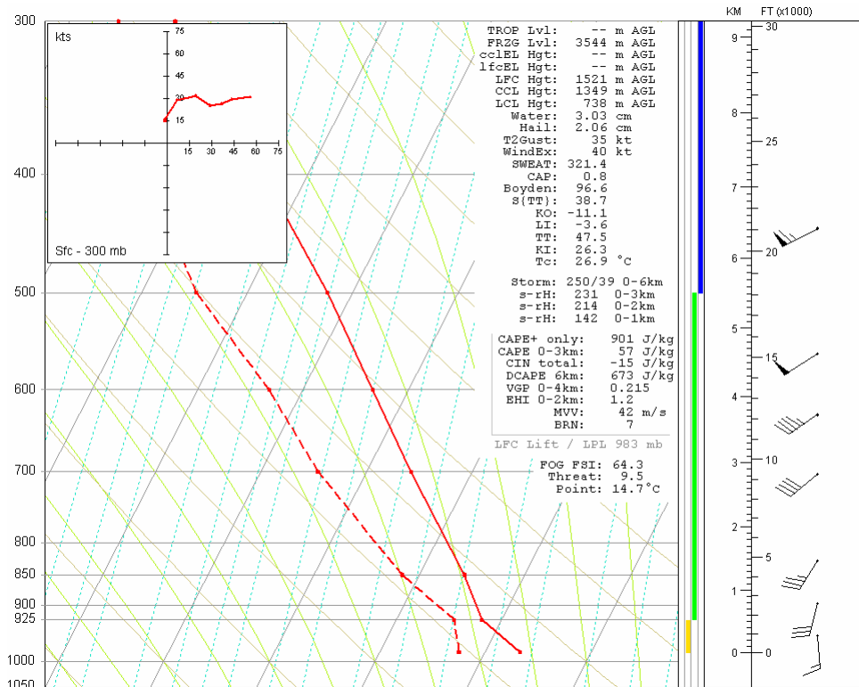
Figure 3. Same as in Fig. 2 except for the Eastern Great Plains (EPL) category.
