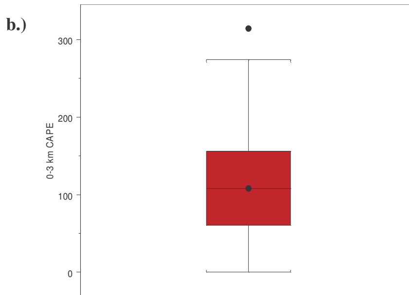
Figure 9. Same as in Fig. 7 except for a) Surface-based CAPE and b) 0-3 km CAPE (J kg -1 ).
