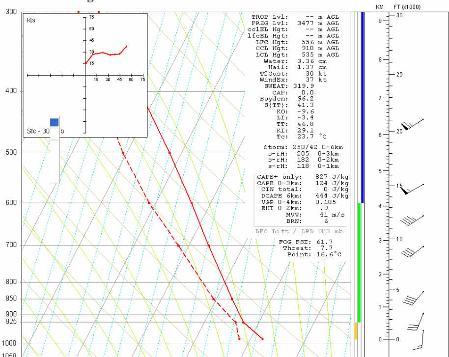
Figure 1. Skew-T/log p diagram representing the composite sounding for the Great Lakes (GRL) ST synoptic category.
