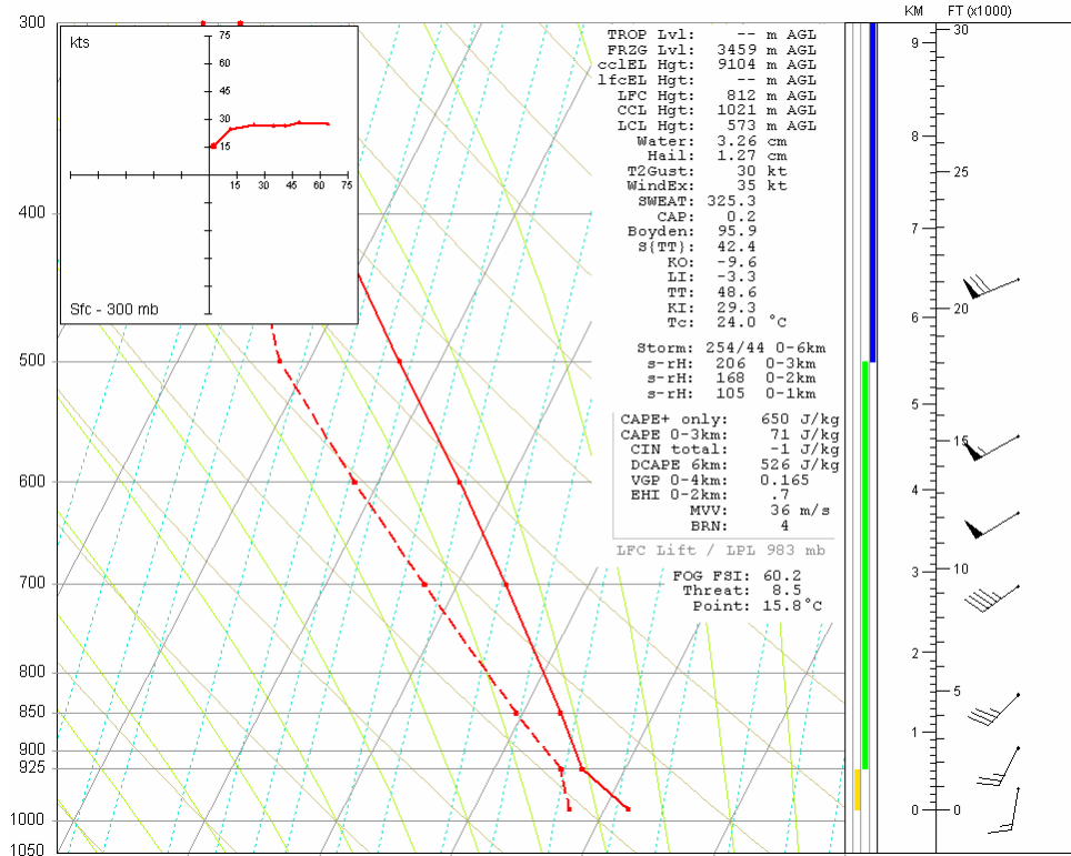
Figure 2. Same as in Fig. 2 except for the Ohio/Tennessee Valley (OTV) composite.
