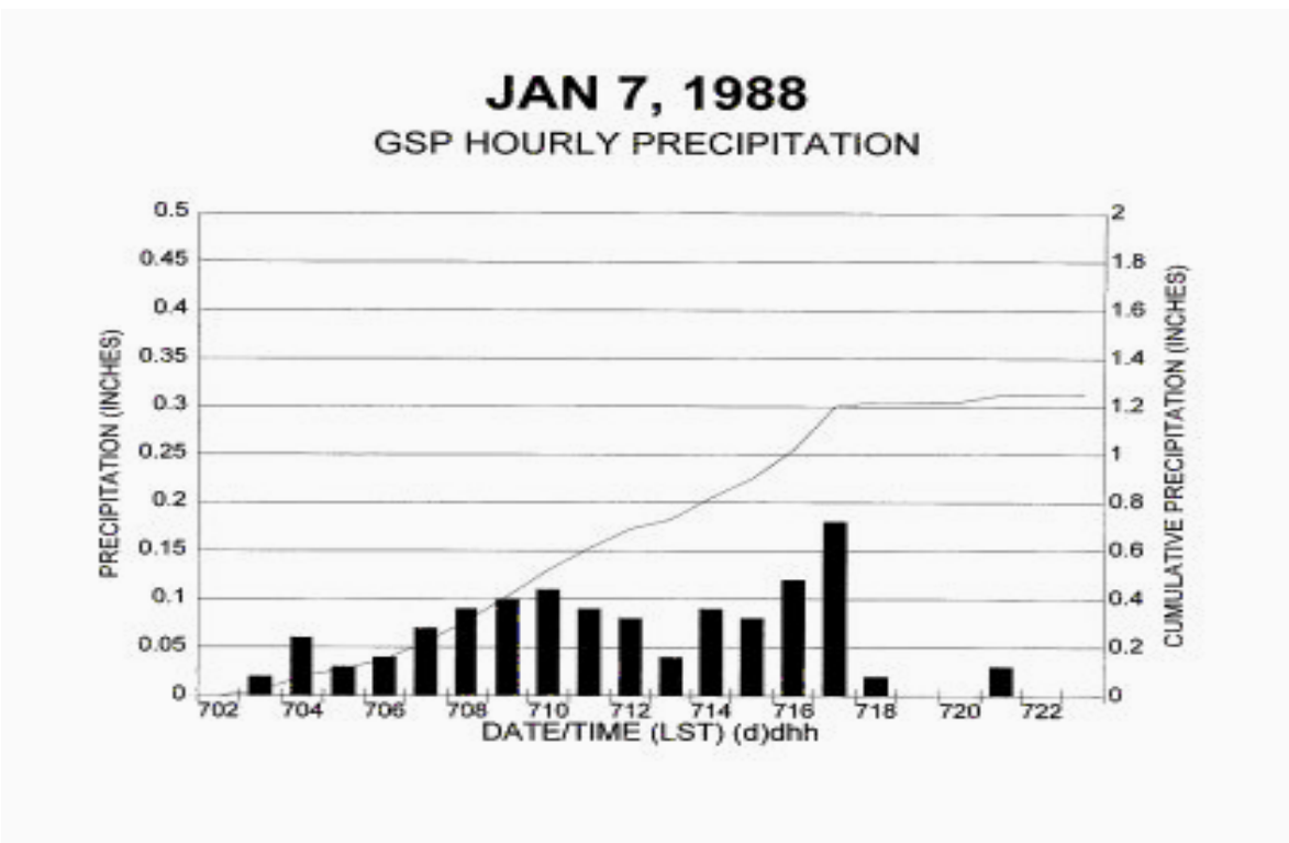
Figure 6. Time series of GSP hourly (columns) and cumulative (line) precipitation in inches from 0200 UTC to 2300 UTC 7 January 1988.
