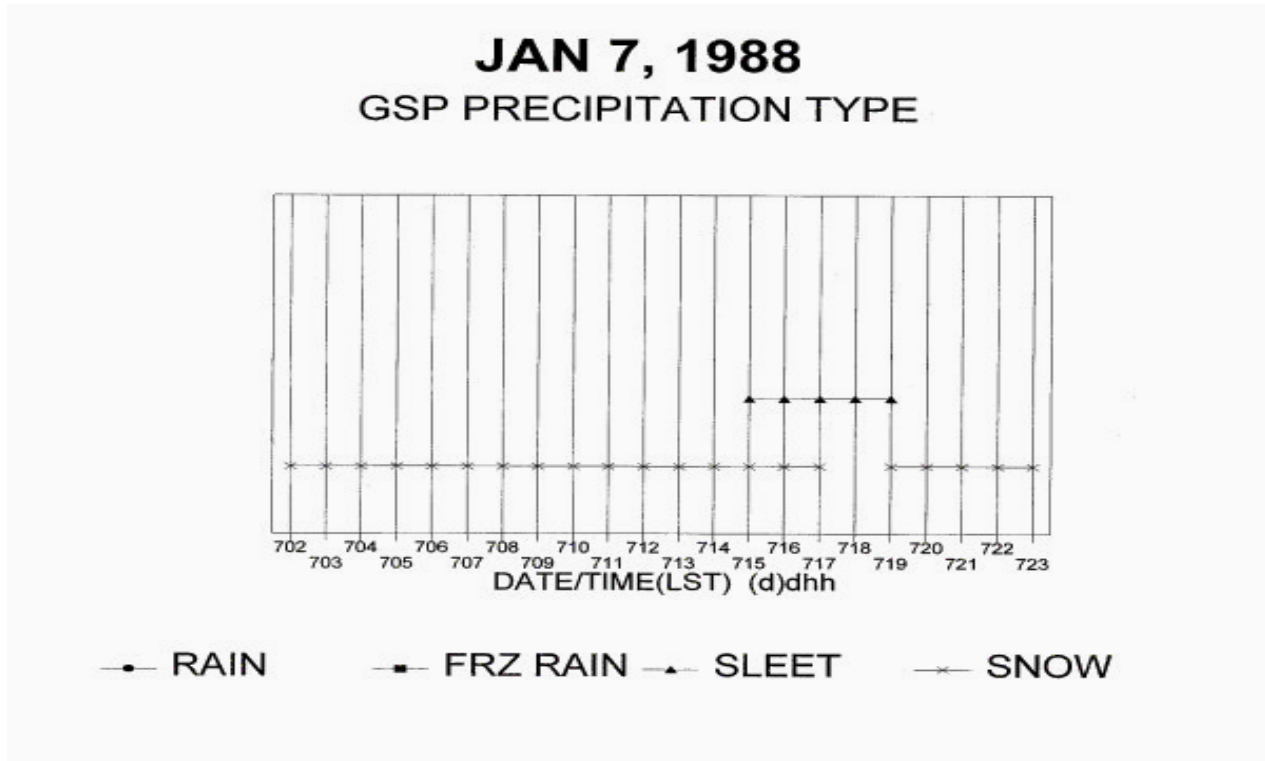
Figure 1. Time series for GSP showing precipitation type observed each hour of the event.
