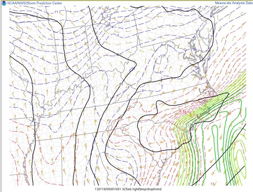
Fig. 16. NOAA/NCEP/SPC mesoanalysis 925 mb height (black contours), temperature (dashed contours), dew point (green contours), and wind (barbs) at 0000 UTC, 18 January 2013.
