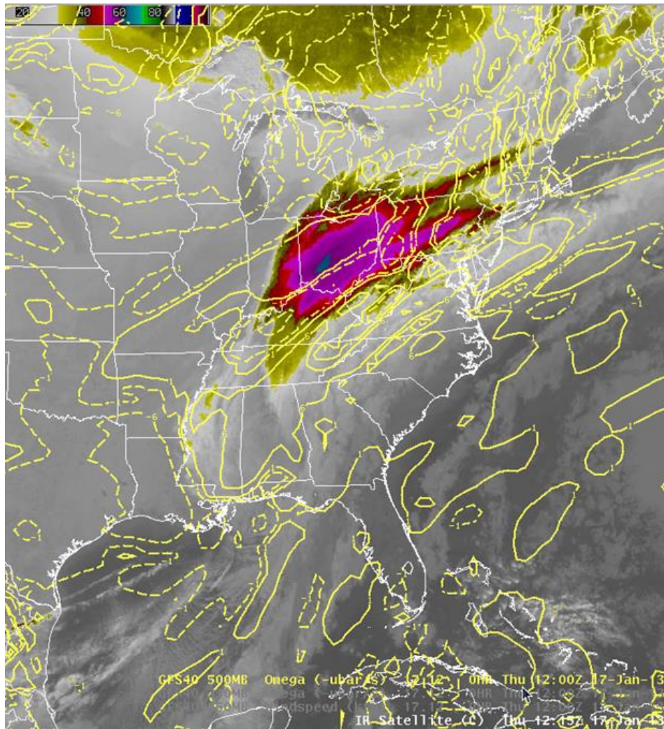
Fig. 7. Same as Fig. 5 except 500 mb omega (microbars \text{sec}^{-1} ; contours).
