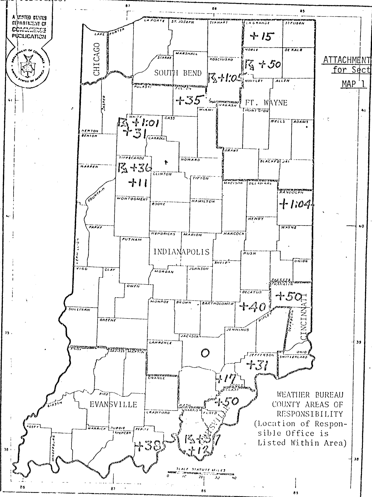
Warning Lead Times in Minutes in Counties where Deaths Occurred on April 3, 1974
