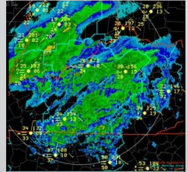
NWS Doppler radar image at 3 am Sunday, February 16 during the height of the ice storm. A surface observation from Lexington showed 30 degrees and freezing rain. Sleet was falling at Louisville, while snow blanketed southwestern Indiana.
