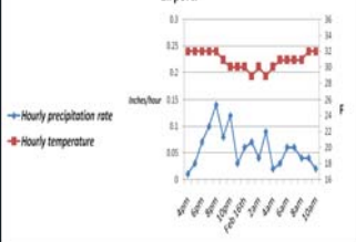
Chart showing temperatures and freezing rain rates from late evening through the morning hours at the Lexington airport.
