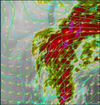
This infrared satellite image shows color-enhanced precipitation producing clouds over the Ohio Valley associated with a deep 500mb trough across Missouri and a strong jet stream over the Tennessee Valley.
