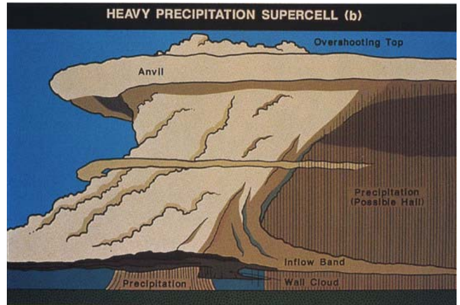
Figure 38: Schematic diagram of a high-precipitation supercell.
