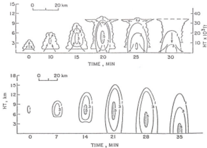
Figure 7: Cloud outlines and radar intensity of a single cell storm (top) and radar intensity of a "pulse" severe storm (bottom).
