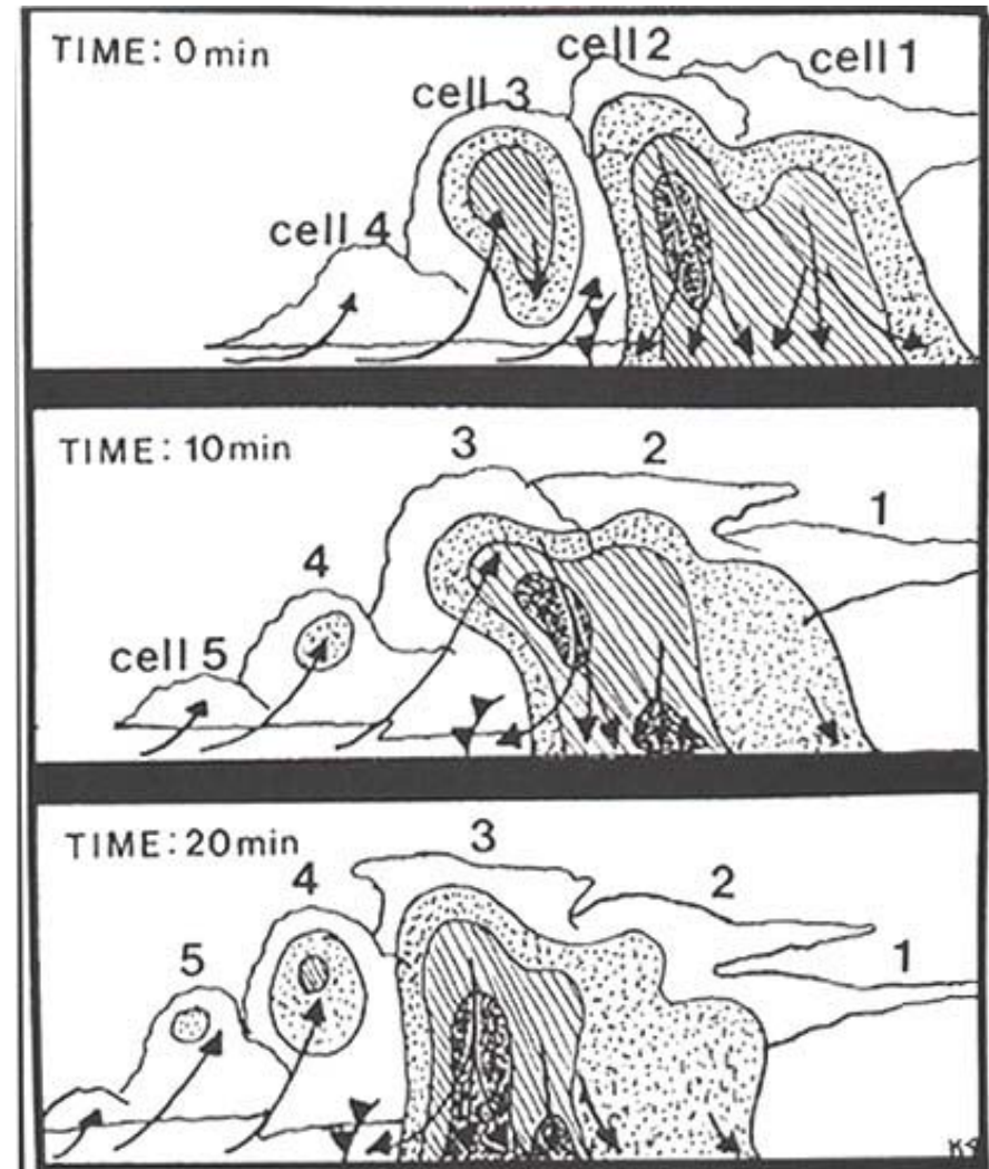
Figure 8: propagation of a multicell cluster storm. Cloud outlines and radar echo intensities are shown.
