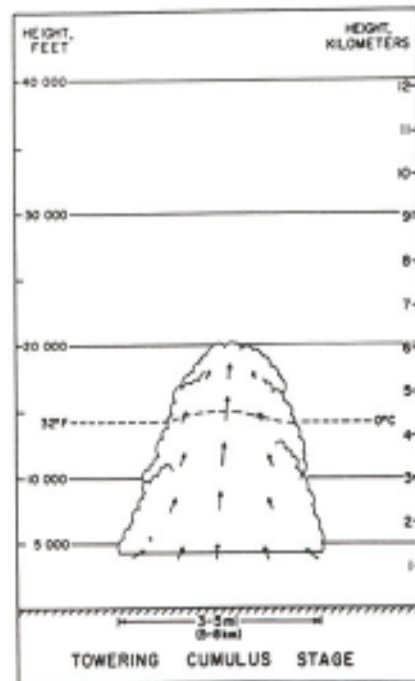
Figure 1: Towering cumulus stage of the thunderstorm. At this time, all air is moving upward in the developing storm.
