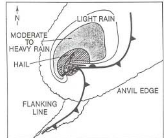
Figure 13: Overhead view of a supercell storm. The precipitation area, gust front, and cloud features are shown.
