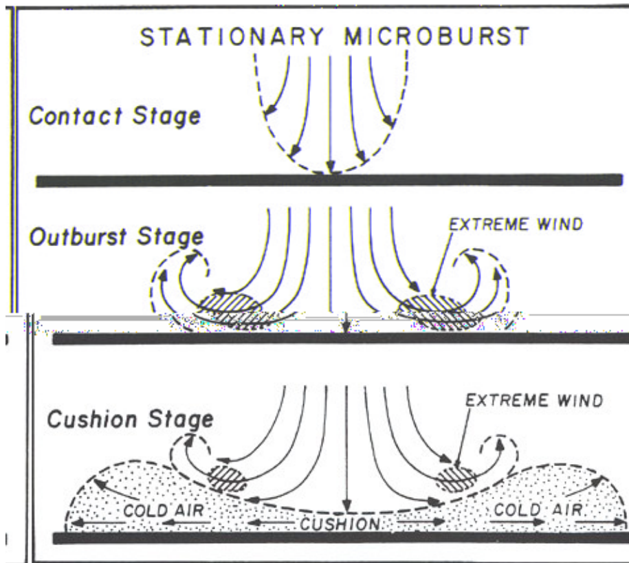
Figure 25. Life cycle of a microburst.
