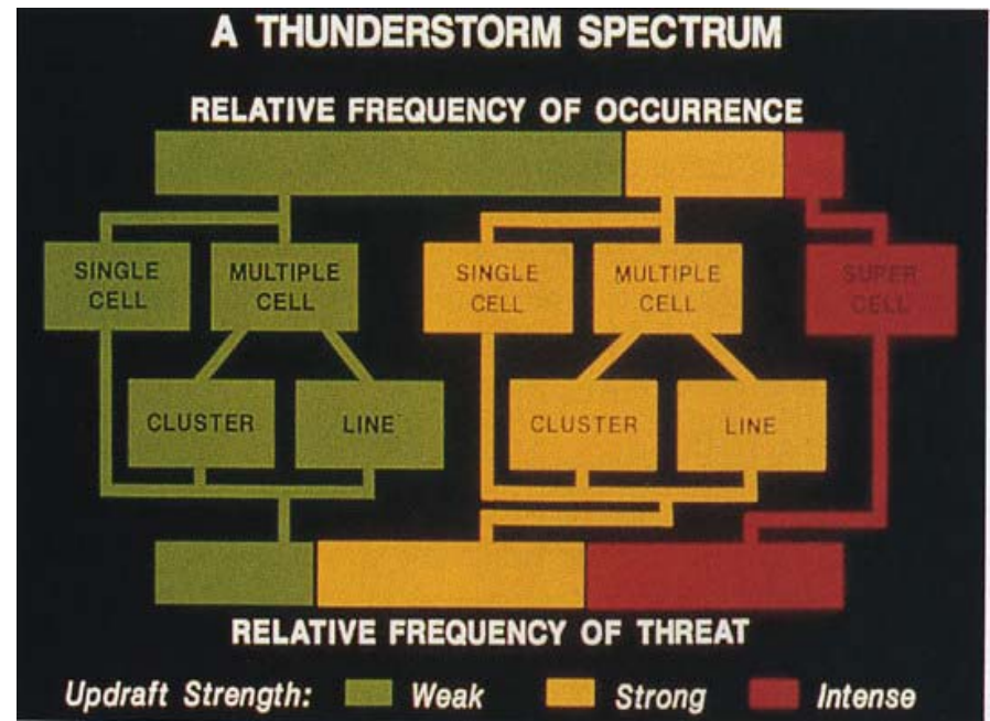
Figure 6: The thunderstorm spectrum. The four main storm categories are listed in the boxes. The bar graphs indicate the frequency and threat with storms of various updraft strength.
