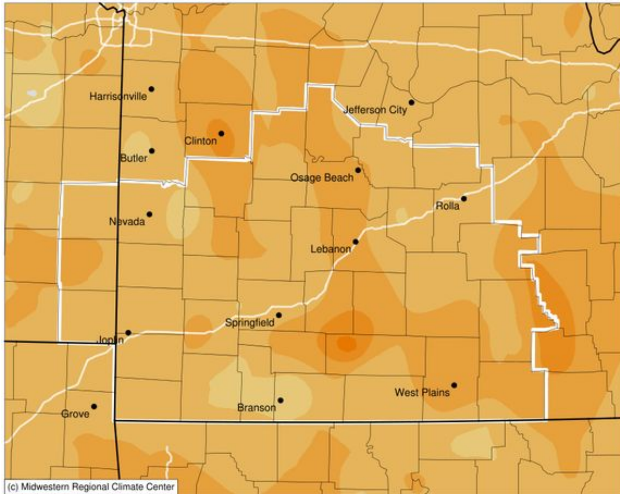
Average Temperature (°F): Departure from 1991-2020 Normals January 01, 2024 to December 31, 2024
