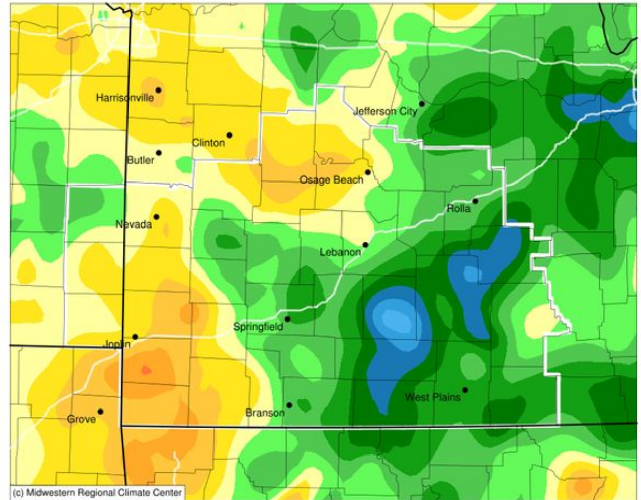
Accumulated Precipitation (in): Departure from 1991-2020 Normals January 01, 2024 to December 31, 2024
