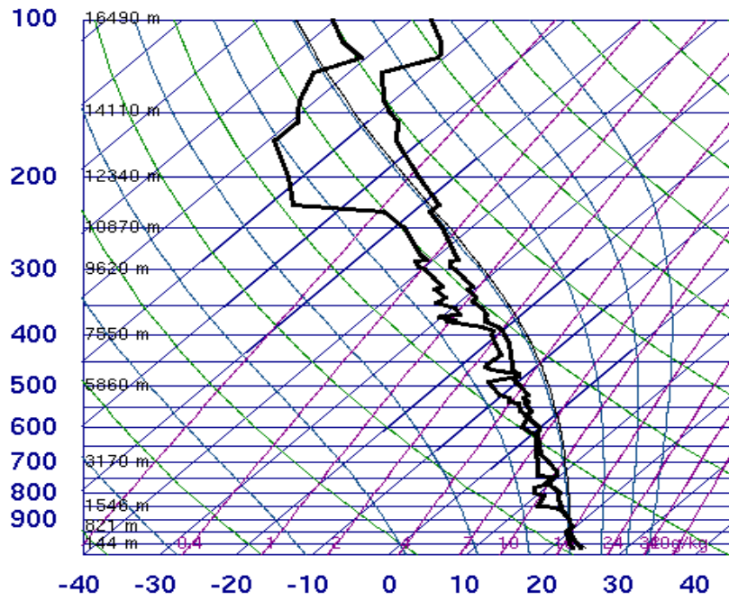
Fig. 13. Upper air sounding for 12 UTC (800 am AST) December 5, 2013 at San Juan, PR, showing 2.19 inches (55.55 mm) of precipitable water.
