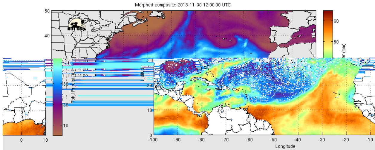
Fig. 4. Precipitable water image for 1200 UTC (800 am AST) on November 30, 2013 ( http://tropic.ssec.wisc.edu/real-time/mimic-tpw/global/main.html )
