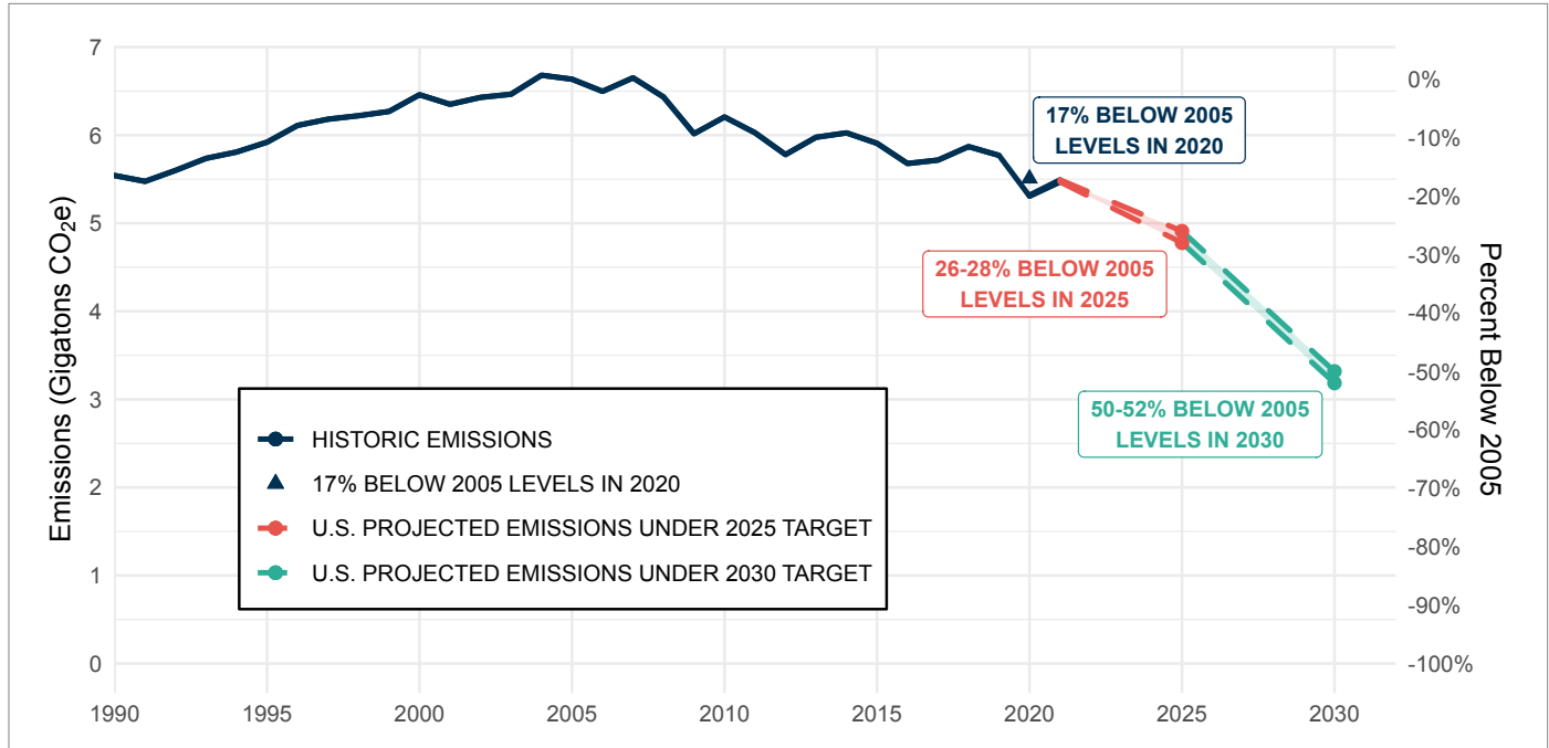
Figure 2: United States historic emissions and projected emissions under the 2030 NDC target.
