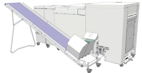
Plockmatic Pro50/35 shown from the back with Trim Waste Conveyor
