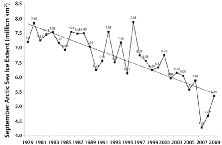
Figure 1. Observed September Arctic sea ice extent decline. Sea ice extent data from the National Snow and Ice Data Center: http://sidads.colorado.edu/DATASETS/NOAA/G02135/ .
