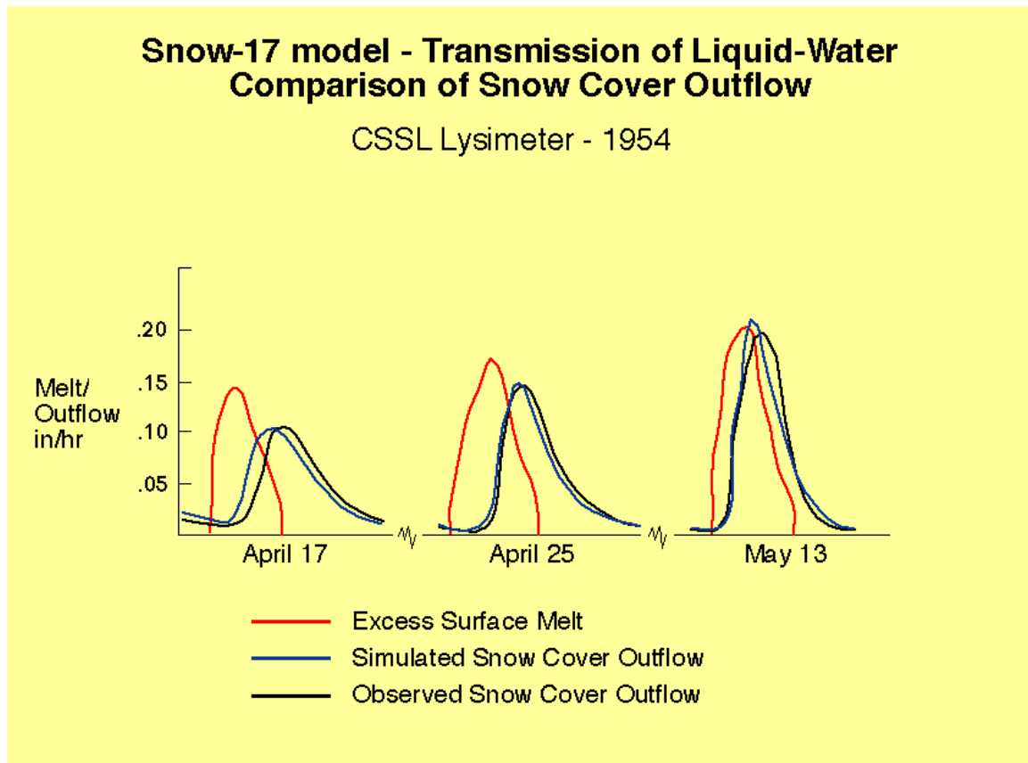
Figure 6. Verification of liquid water transmission algorithms.
