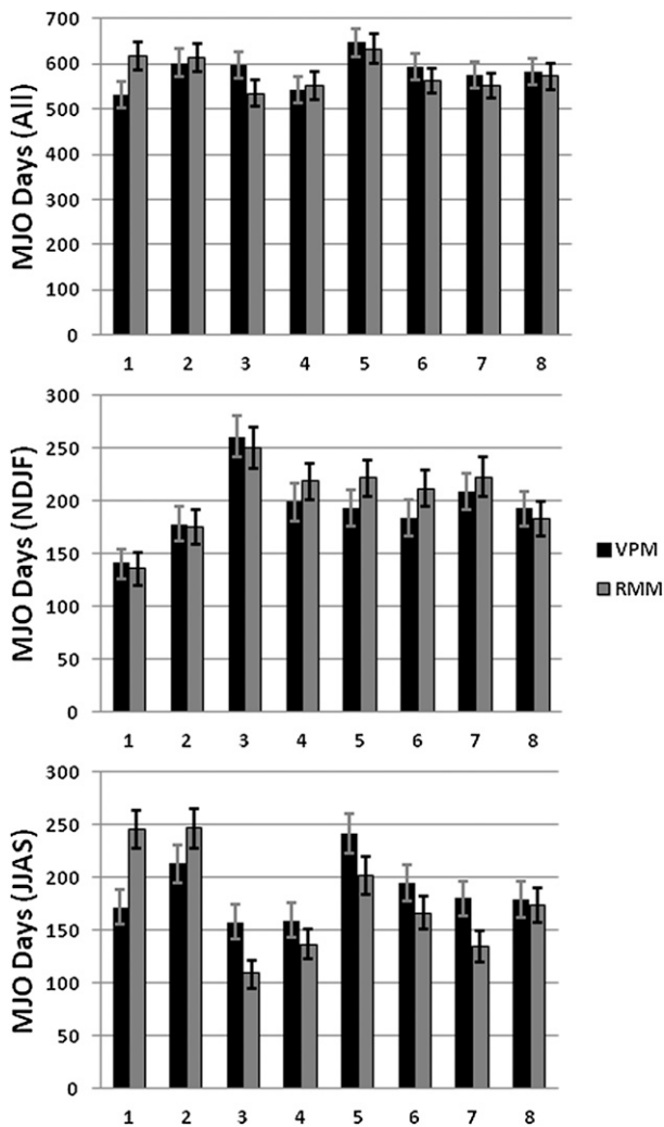
FIG. 6. The number of MJO days, defined as a day where the amplitude for the VPM (black) or RMM (gray) index was greater than or equal to one standard deviation, binned for all MJO phases during (top) all months; (middle) boreal winter (November–February) only months; and (bottom) boreal summer (June–September) only months. The 90% confidence interval is indicated by the error bars.
