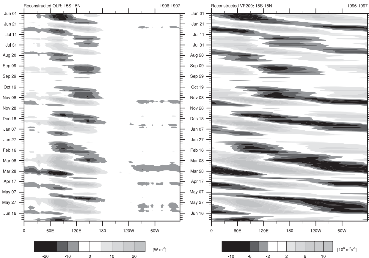
FIG. 5. Time-longitude plots of (left) reconstructed OLR and (right) reconstructed VP200 from the leading EOF pair of the VPM EOF analysis for the period between June 1996 and June 1997.
