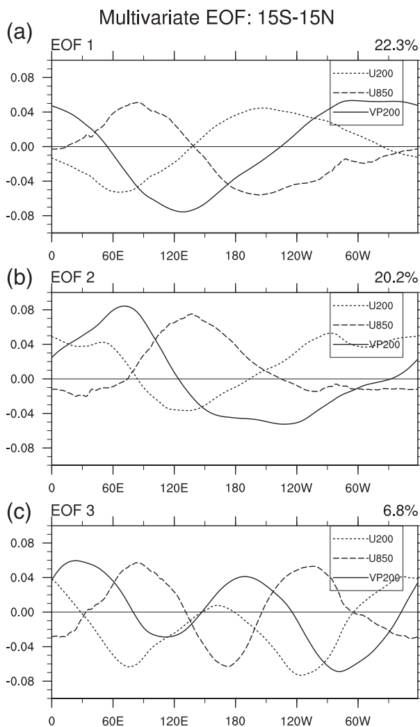
FIG. 1. Spatial structures of EOFs 1, 2, and 3 of the combined analysis of anomalous U200, U850, and VP200. EOFs are constructed by using data averaged over 15°S–15°N, including all longitudes. Magnitudes are plotted on the same relative axis. The variance explained by the respective EOFs is 22.3%, 20.2%, and 6.8%, respectively.
