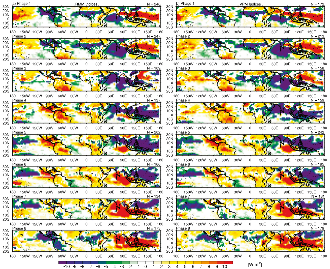
FIG. 8. JJAS composite of anomalous OLR (shaded) for each MJO phase using (a) the RMM PCs and (b) the VPM PCs using VP200 instead of OLR. Anomalies statistically different than zero at the 90% level are shaded.
