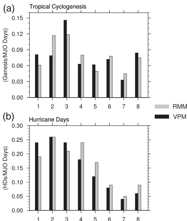
FIG. 9. (a) Normalized Atlantic genesis days and (b) normalized Atlantic hurricane days (HDs) for each MJO phase for the VPM PCs (black) and the RMM PCs (gray) during the JJAS (1989–2009) season. Both (a) and (b) are normalized by the number of MJO days for each particular MJO phase.
