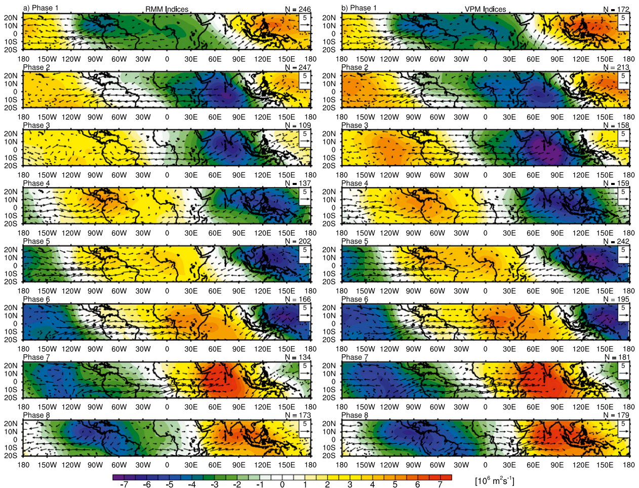
FIG. 7. JJAS composite of anomalous VP200 (shaded) and 200-hPa wind anomalies (vectors) for each phase using (a) the RMM PCs and (b) the VPM PCs. VP200 anomalies statistically different than zero at the 95% level are shaded. Negative VP200 anomalies represent upper-level divergence. The number of days in each phase N is provided. The reference vector is 5 \text{ m s}^{-1} .
