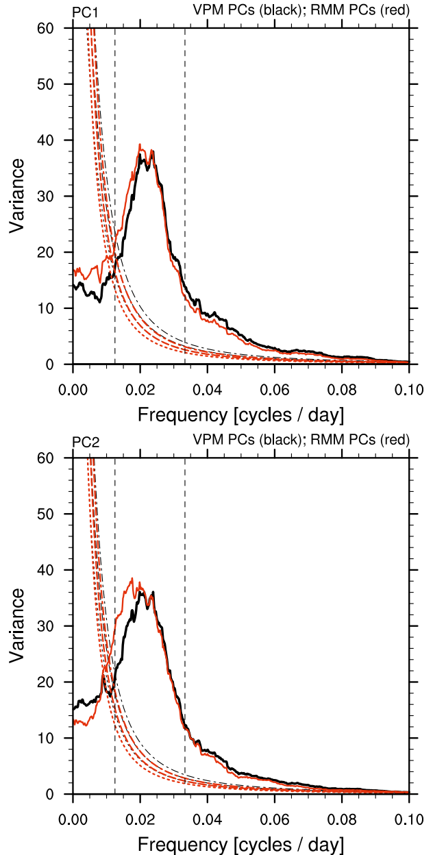
FIG. 2. Power spectra of the PCs for the leading two EOFs of combined fields shown of Fig. 1. The original EOFs from WH04 are also included and indicated by the red line. The curved-dashed black and red lines represent the red-noise spectrum for the VPM PCs and RMM PCs, respectively. The upper limit represents the 95% confidence interval and the lower limit represents the 5% confidence interval. The two vertical dashed lines represent the 30–80-day range.
