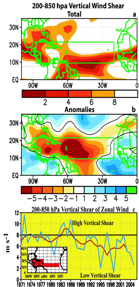
Fig. 4. 200-850 hPa vertical shear magnitude (a) total ( \text{m s}^{-1} ) and (b) anomalies during June-October 2005. In (a) only values less than 8 \text{ m s}^{-1} are shaded. In (b) red shading indicates weaker-than-average vertical shear. Green box denotes the MDR. Anomalies in (b) are departures from the 1971-2000 base period monthly means.
