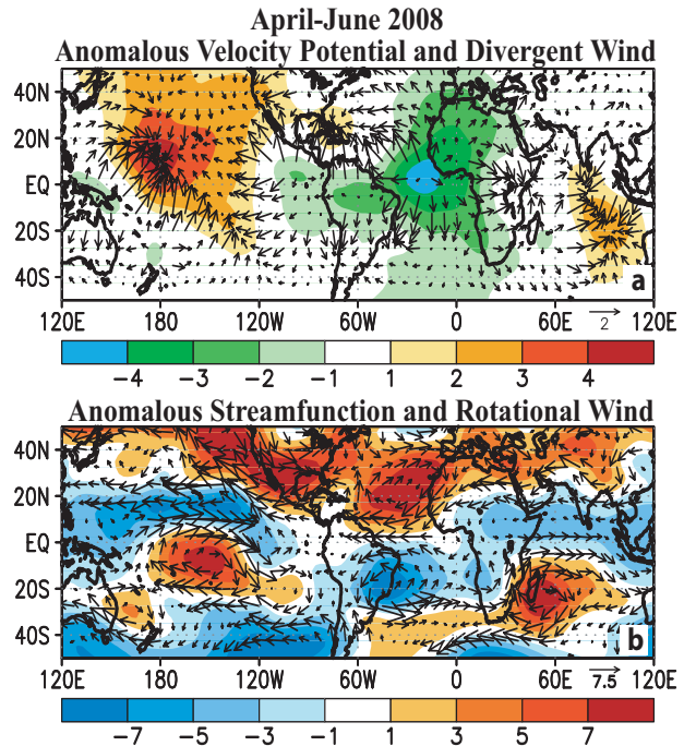
Fig. 11. Apr-Jun 2008 anomalies at 200-hPa: (a) velocity potential (shading) and divergent wind vectors ( m s^{-1} ), and (b) streamfunction and total wind vectors ( m s^{-1} ). In (b) anomalous ridges are indicated by positive values (red) in the NH and negative values (blue) in the SH. Anomalous troughs are indicated by negative values in the NH and positive values in the SH. Anomalies are departures from the 1971-2000 monthly means.
