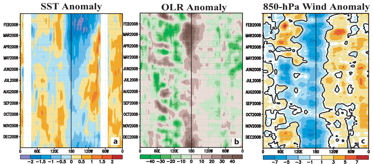
Fig. 10. Equatorial time longitude sections of anomalies averaged between 5N-5S: (a) weekly sea surface temperatures ( ^{\circ}\text{C} ), (b) Outgoing Longwave Radiation (OLR, \text{W m}^{-2} ), and (c) 850-hPa zonal winds ( \text{m s}^{-1} ). In (b) brown shading shows suppressed convection and green shading shows enhanced convection. In (c) blue shading shows easterly anomalies and orange shading shows westerly anomalies. Anomalies are departures from the (a) 1971-2000 weekly SST means, (b) 1979-2000 pentad OLR means, and (c) 1971-2000 pentad zonal wind means. A 3-pt running mean is applied to the data in all plots.
