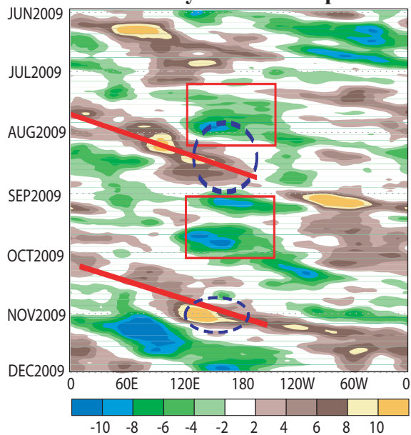
Fig. 10. Time-longitude section showing departures of 200-hPa velocity potential averaged between 5°N-5°S. For each day, the average departure for the previous 120 days is removed prior to plotting. Green (brown) shading highlights likely areas of anomalous divergence and rising motion (convergence and sinking motion). Red lines highlight the main MJO episodes. Anomalies are departures from the 1971-2000 base period daily means.
