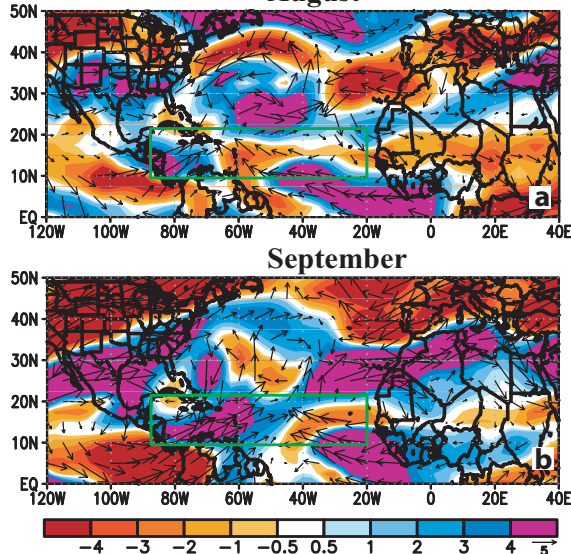
Fig. 11. Departures from normal of 200-850 hPa vertical wind shear magnitude ( m s^{-1} ) and vectors during (a) August 2009 and (b) September 2009. Green box denotes the MDR. Vector scale is to right of color bar. Anomalies are departures from the 1971-2000 period monthly means.
