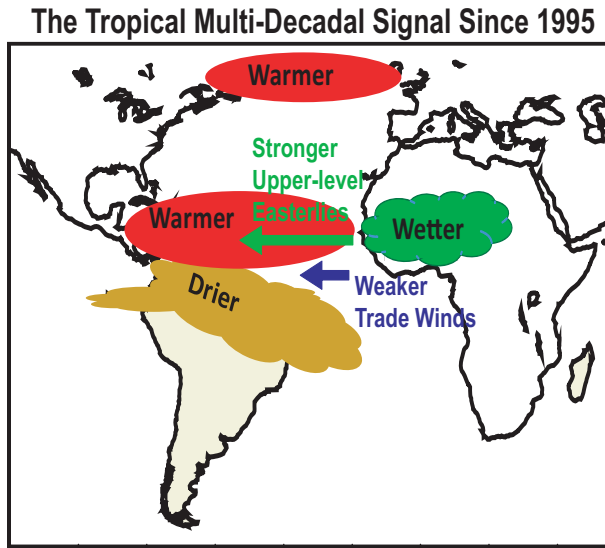
Fig. 13. Schematic depiction of the tropical multi-decadal signal during 1995-2011, adapted from Bell and Chelliah (2006).
