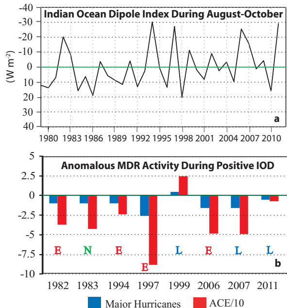
Fig. 16. (Top) ASO time series of the Indian Ocean Dipole (IOD), calculated as the difference in area-averaged OLR anomalies ( \text{W m}^{-2} ) between the western and eastern Indian Ocean (western minus eastern, boxes shown in Fig. 11). Anomalies are with respect to the 1981-2010 period monthly means. (Bottom) Anomalous Atlantic major hurricane (blue) and ACE/10 (i.e., \times 10^3 \text{ kt}^2 ) activity associated with storms first named in the MDR when there was a strong positive IOD during ASO. Anomalies for years during 1979-1994 (low-activity era) and 1995-2011 (high-activity era) are based on the respective period means. Corresponding El Niño (red E), La Niña (blue L), and ENSO-Neutral (green N) periods are indicated.
