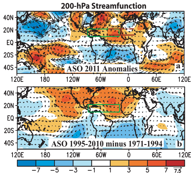
Fig. 9. 200-hPa streamfunction (shading, \times 10^6 \text{ m}^2 \text{ s}^{-1} ) and wind vectors ( \text{m s}^{-1} ): (a) Anomalies during ASO 2011 and (b) difference between 1995-2010 and 1971-1994 ASO means. In (a), brown solid (dashed) line over the eastern MDR shows location of mean ridge axis during ASO 2011 (ASO 1995-2010). Anomalous ridges are indicated by positive values (red) in the NH and negative values (blue) in the SH. Anomalous troughs are indicated by negative values in the NH and positive values in the SH. Green boxes denote the MDR. Vector scale is below right of color bar. Anomalies are with respect to the 1981-2010 period monthly means.
