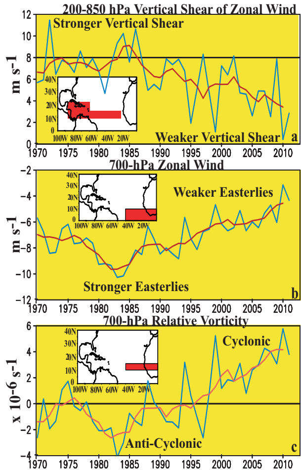
Fig. 14. Time series showing consecutive ASO values of area-averaged (a) 200-850 hPa vertical shear of the zonal wind ( \text{m s}^{-1} ), (b) 700-hPa zonal wind ( \text{m s}^{-1} ) and (c) 700-hPa relative vorticity ( \times 10^{-6} \text{ s}^{-1} ). Blue curve shows unsmoothed values, and red curve shows a 5-pt running mean of the time series. Averaging regions are shown in the insets.
