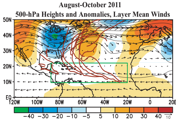
Fig. 4. ASO 2011: 500-hPa heights (contours, m) and anomalies (shading), and layer mean wind vectors ( \text{ms}^{-1} ) between 600 hPa – 300 hPa. Atlantic named storm tracks are shown in brown. Green box denotes the MDR. Vector scale is below right of color bar. Anomalies are with respect to the 1981-2010 period monthly means.
