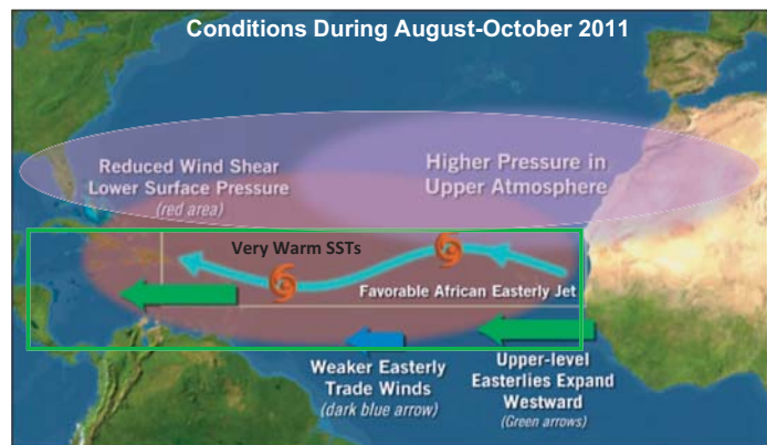
Fig. 7. Conditions over the Atlantic basin during ASO 2011. Green box denotes the Main Development Region (MDR).
