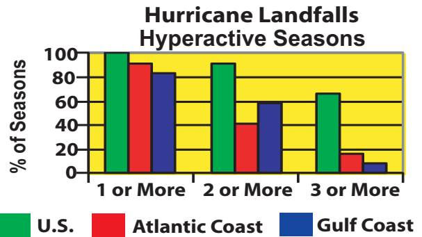
Fig. 5. Seasonal frequency (during 1950-2009) of Atlantic basin hurricanes making landfall in the United States during hyperactive seasons. Green bars show landfalls for the entire U.S., red bars show landfalls along the U.S. Atlantic Coast, and blue bars show landfalls along the U.S. Gulf Coast. Landfalls are based on the HURDAT data produced by the National Hurricane Center and compiled by Blake et al. (2011).
