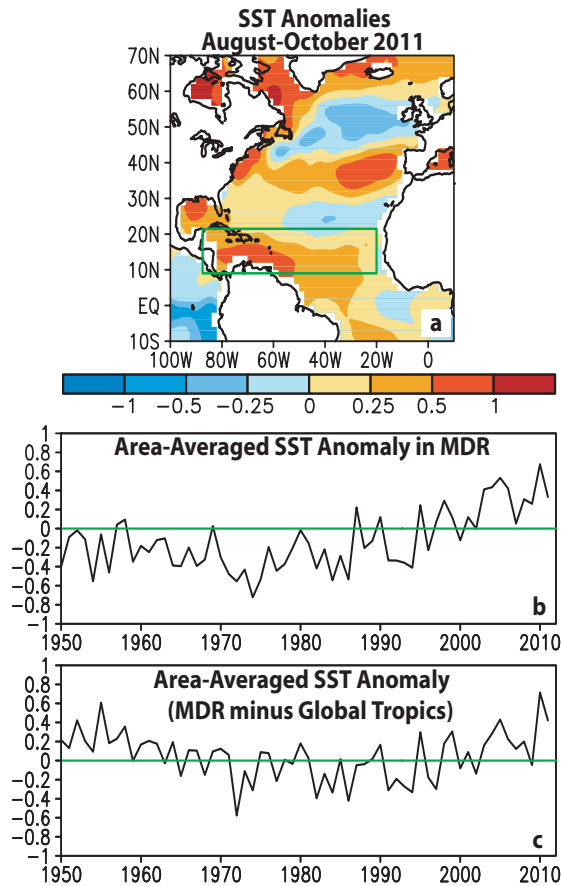
Fig. 6. (a) ASO 2011 sea surface temperature (SST) anomalies ( ^{\circ}\text{C} ). (b) Time series of consecutive ASO area-averaged SST anomalies ( ^{\circ}\text{C} ) in the MDR [green box in (a)]. (c) Time series showing the difference between ASO area-averaged SST anomalies ( ^{\circ}\text{C} ) in the MDR and those for the entire global tropics ( 30^{\circ}\text{N} - 30^{\circ}\text{S} ). Anomalies are departures from the ERSST-v3b (Smith et al. 2008) 1981-2010 period monthly means.
