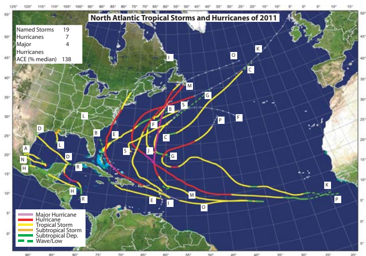
Fig. 1. Tracks of Atlantic named storms during 2011. Storm intensity is color-coded as indicated at bottom left. Letters correspond to the first initial of the storm name.
