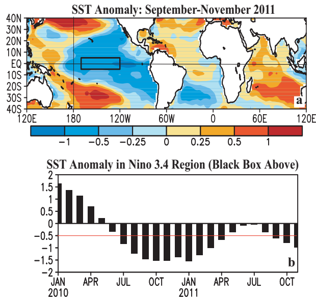
Fig. 15. (a) Sep.-Nov. 2011 sea surface temperature (SST) anomalies ( ^{\circ}\text{C} ). (b) Time series of monthly area-averaged SST anomalies in the Niño 3.4 region [black box in (a)], with red line indicating the threshold for a La Niña. Anomalies are departures from the ERSST-V3b (Smith et al. 2008) 1981-2010 period monthly means.
