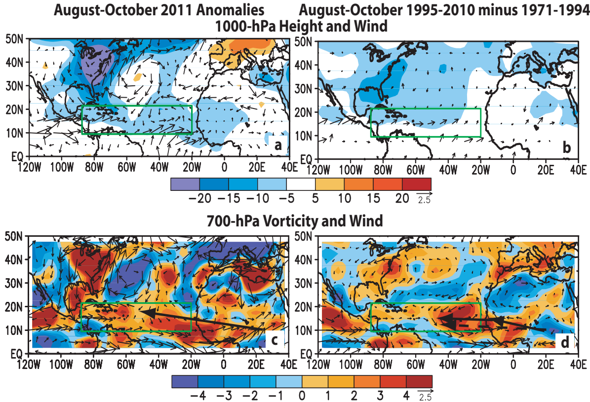
Fig. 8. (Left) ASO 2011 anomalies and (Right) difference between the 1995-2010 and 1971-1994 ASO means. Panels (a, b) show 1000-hPa heights (shading, m) and wind vectors ( \text{m s}^{-1} ). Panels (c, d) show 700-hPa relative vorticity (shading, \times 10^{-6} \text{ s}^{-1} ) and wind vectors. In (c) thick arrow shows the axis of the African easterly jet (AEJ). In (d) thick solid (dashed) arrow indicates the mean position of the AEJ during 1995-2010 (1971-1994). Vector scales are below right of color bars. Green boxes denote the MDR. Anomalies are with respect to the 1981-2010 period monthly means.
