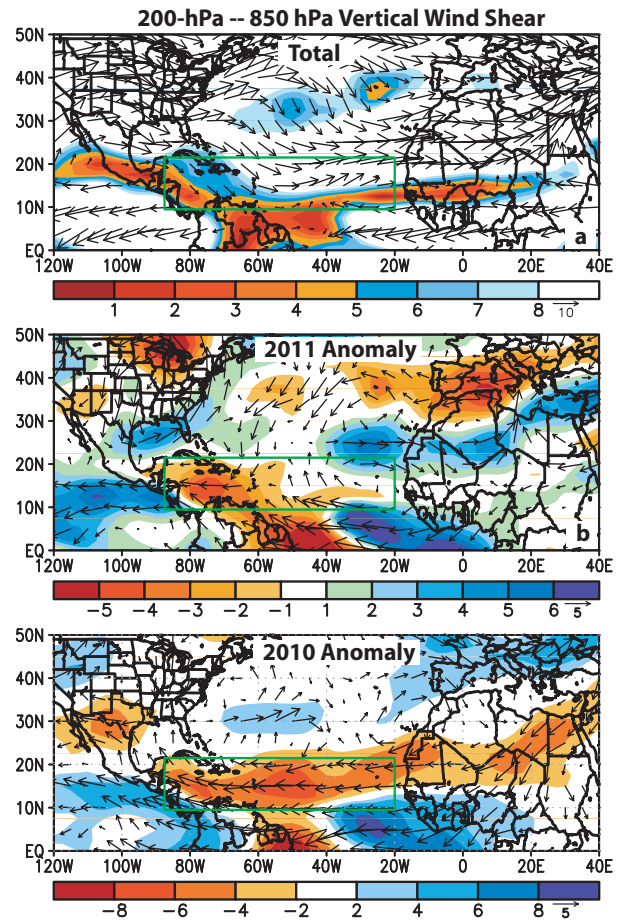
Fig. 10. ASO 2011 vertical wind shear magnitudes and vectors ( \text{m s}^{-1} ): (a) total and (b) anomalies. Panel (c) shows corresponding shear anomalies for ASO 2010. Green boxes denote the MDR. Vector scales are below right of color bars. Anomalies are with respect to the 1981-2010 period monthly means.
