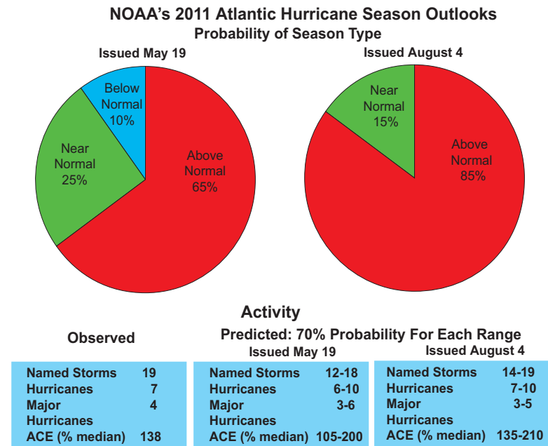
Fig. 3. NOAA's 2011 Atlantic hurricane season outlooks issued on 19 May and updated on 4 August. The observed seasonal activity is also indicated.
