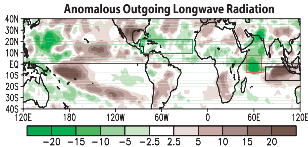
Fig. 11. ASO 2011 anomalous Outgoing Longwave Radiation (OLR, \text{W m}^{-2} ). Red (black) box denotes the western (eastern) portion of the Indian Ocean dipole (IOD). Green box denotes the MDR. Anomalies are with respect to the 1981-2010 period monthly means.
