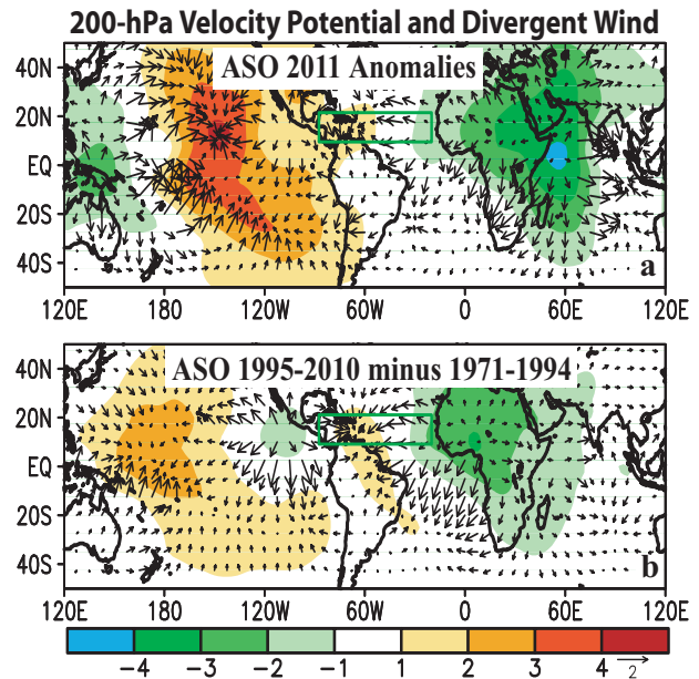
Fig. 12. 200-hPa velocity potential (shaded, \times 10^6 \text{ m}^2 \text{ s}^{-1} ) and divergent wind vectors ( \text{m s}^{-1} ): (a) ASO 2011 anomalies, and (b) difference between the 1995-2010 and 1971-1994 ASO means. Green boxes denote the MDR. Vector scale is below right of color bar. Departures are with respect to the 1981-2010 period monthly means.
