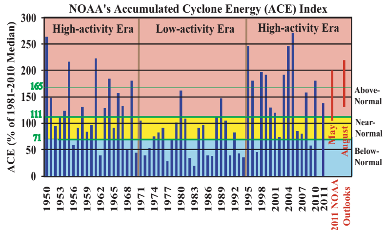
Fig. 2. NOAA's Accumulated Cyclone Energy (ACE) index expressed as percent of the 1981-2010 median value. ACE is calculated by summing the squares of the 6-hourly maximum sustained wind speed (knots) for all periods while the storm has at least tropical storm strength. Red bars show NOAA's predicted ACE ranges in their May and August seasonal hurricane outlooks. Pink, yellow, and blue shadings correspond to NOAA's classifications for above-, near-, and below-normal seasons, respectively. The 165% threshold for a hyperactive season is indicated. Vertical brown lines separate high- and low-activity eras.
