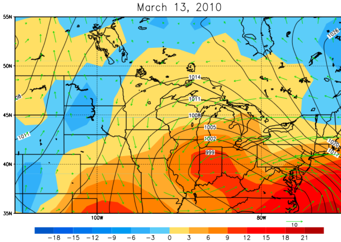
Figure 1. Air temperature (shaded, C), surface winds (vectors, m/s) and sea level pressure (contours, hPa) on March 13-14, 2010, and February 13-14 showing the passage of a cyclone from west to east. The data are from NCEP2. ( www.cpc.ncep.noaa.gov/products/wesley/reanalysis2/ )
