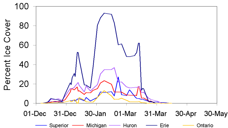
Figure 13. Daily lake-averaged ice cover winter 2010.
