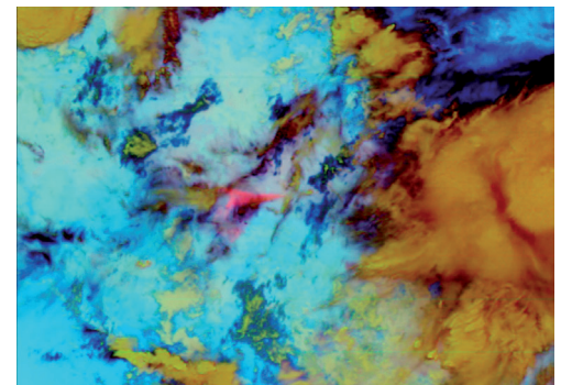
Volcanic ash from the September 27, 2017, eruption of the Popocatepetl volcano in Mexico was detected by GOES-16. The reddish pink colors indicate ash. The other colors denote the following: yellowish/brown colors are thick clouds, the dark blues are thin cirrus clouds, and the pale blue indicates the surface (land and water) of the Earth. Credit: NOAA/CIRA
