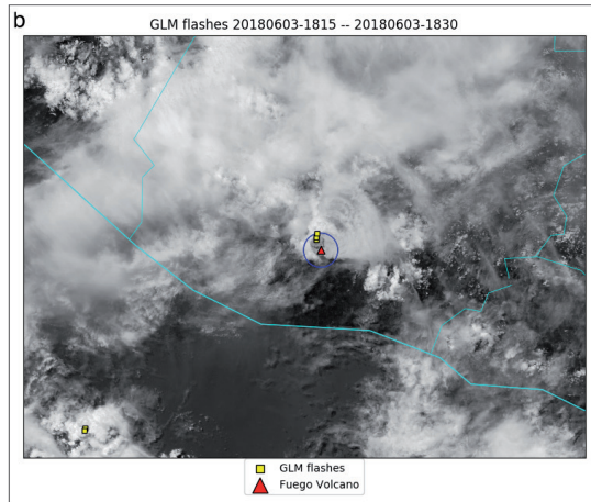
GOES-16 ABI visible imagery from June 3, 2018, of the Fuego Volcano eruption with GLM lightning data overlaid (yellow squares) in the area circled on the image. Credit: NOAA/CIMSS
