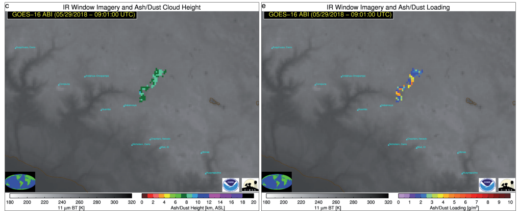
GOES-16 VOLCAT ash height (left) and ash mass loading (right) from the Sabancaya Volcano eruption in Peru on May 29, 2018. Credit: NOAA/CIMSS
