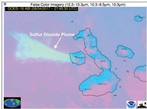
GOES-16 false color ash RGB image of the Fernandina volcano in the Galápagos Islands on September 4, 2017. This volcanic plume was rich in SO 2 , depicted as a green plume in this imagery. Credit: NOAA/CIMSS
