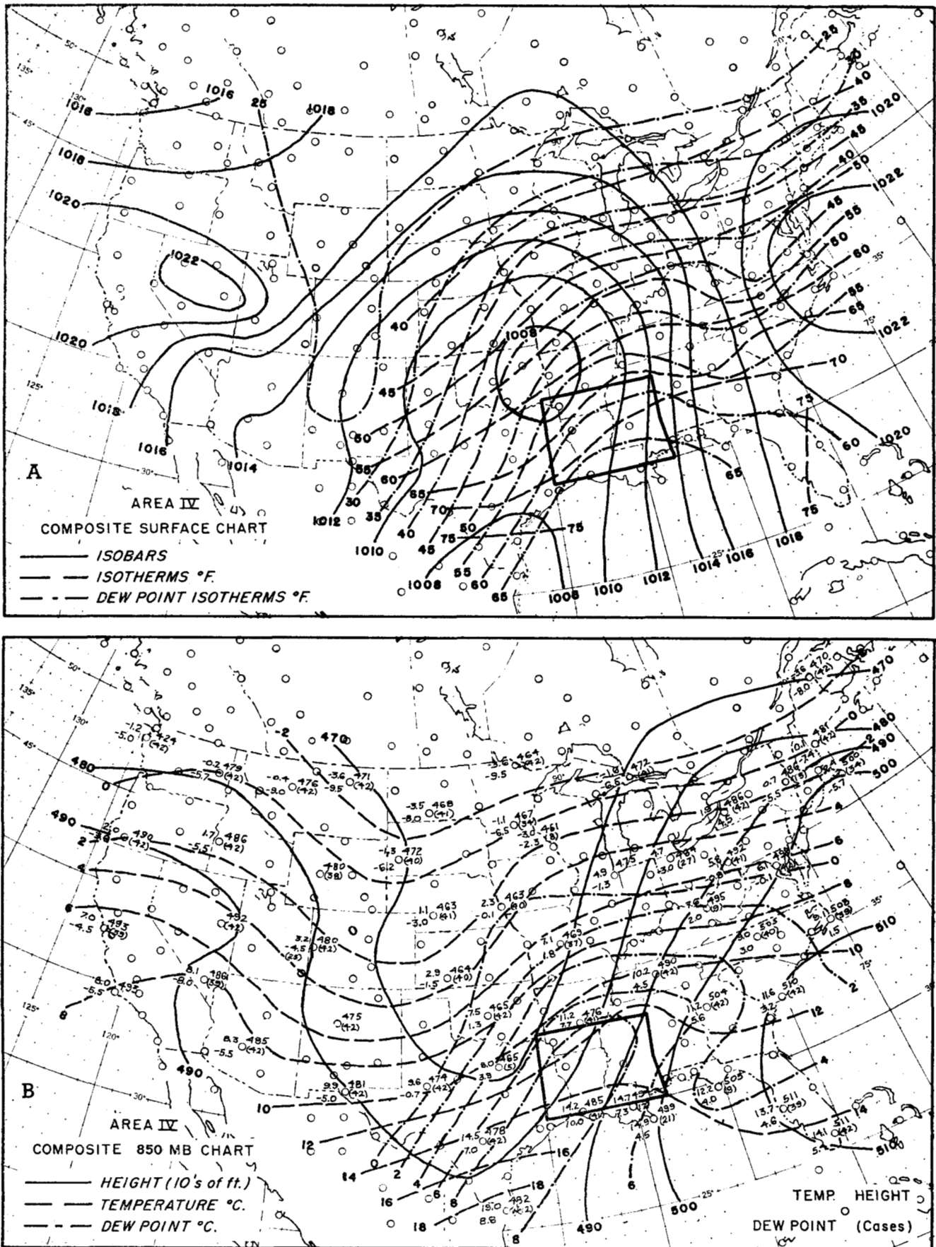
FIGURE 5.—Composite maps from 42 tornado situations (191 tornadoes) that occurred in area IV from January through May 1945 through 1953. (A) Surface, (B) 850 mb., (C) 700 mb., (D) 500 mb.
