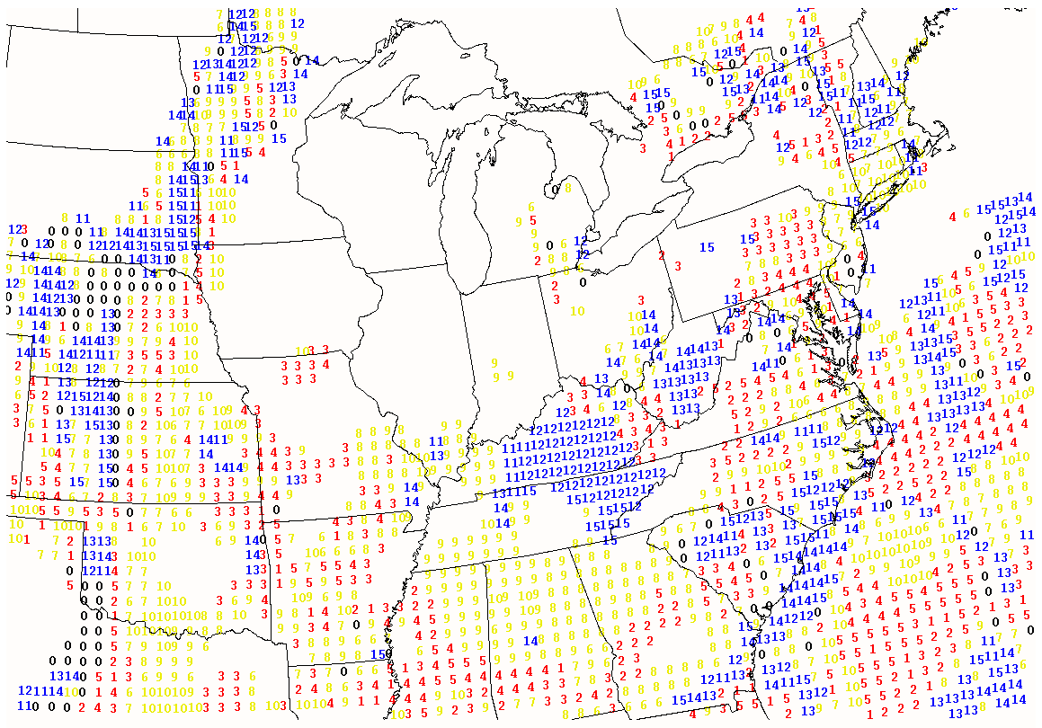
NCEP_SREF 030528/0000V015 2 M BEST MEMBER SFC Td >= 50F (0=Mean; 1-15 Mems; Mean=White; Eta=Reds; KFs=Yellows; RSM=Blues) Fig. 7: The NCEP SREF ensemble member closest to the RUC analysis valid at 00 UTC 28 May 2003. (Black 0 indicates the ensemble mean; Yellow=Eta-BMJ members; Red=Eta-KF members; and Blue=RSM members)
