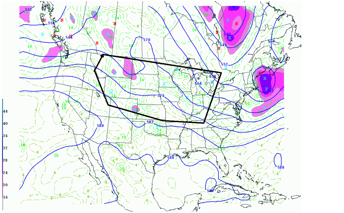
RUC2A 030602/0000 500 MB HEIGHTS AND ABS VORTICITY (*10**5) Fig. 8: Domain considered (black, solid line) for determining the best NCEP SREF ensemble member from the 09 UTC 01 June 2003 case. The 500 hPa geopotential height (solid) and absolute vorticity (dashed) are from the RUC analysis valid at 00 UTC 02 June 2003.
