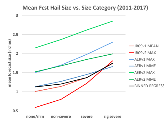
Figure 8 Same as Fig. 5, but relative to MESH. Result from binned regression based on CAPE and 0-6 km shear is shown in black.
