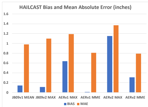
Figure 4 Bias (blue) and RMSE (orange) relative to “ground truth” hail size reports for different versions of HAILCAST
