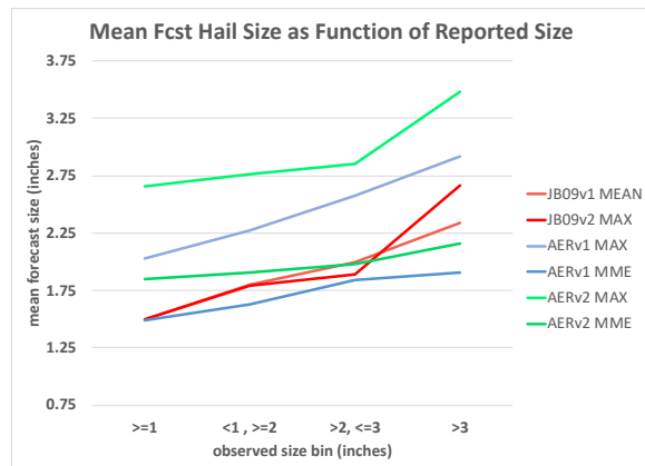
Figure 5 Mean forecast size as a function of “ground truth” hail size bin for different versions of HAILCAST
