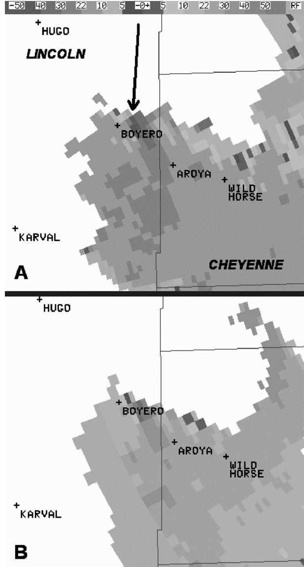
FIG. 5. The 0.5° elevation angle SRM displays at 0034 UTC 16 Jun 2002, from (a) PUX and (b) GLD. County names, arrow pointing toward mesoanticyclone center, and the velocity grayscale each are provided in (a). Locality names appear on both images, which are scaled identically. PUX and GLD radars were located generally southwest of (a) and northeast of (b), respectively. Velocities are shown in kt (1 kt ≈ 0.5144 m s -1 ).
