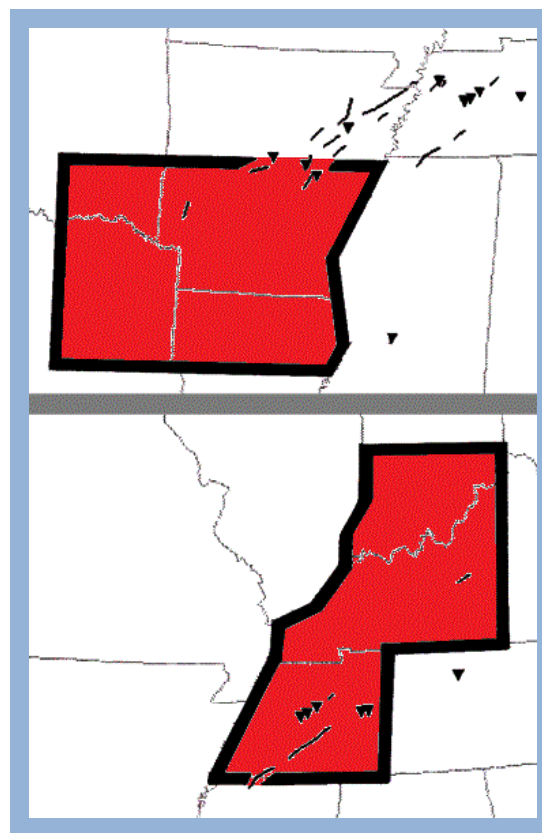
Figure 2: Areal outline (black) and coverage (red) of the first successful SWU tornado "bulletins" (watches). Top: 1800 UTC 21 March 1952; bottom: 0330 UTC 22 March 1952. Triangles and paths denote tornado locations during valid times. Adapted from Fig. 4 of Corfidi (1999).
