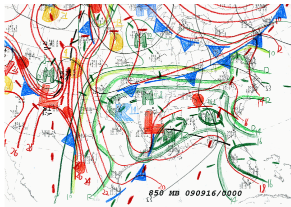
Figure 4: Example of operational SPC hand analysis on an 850-hPa chart, 0000 UTC 16 September 2009, with conventional synoptic features drawn. Isohypsers in black (dam), isotherms in red (°C), isodrosotherms in green (°C), dewpoint maxima (minima) marked “M” (“D”). Thermal minimum marked “K”. Moist (green) and thermal (red) axes represented by thick, loosely dashed lines.
