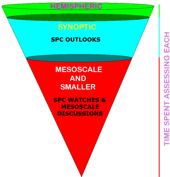
Figure 5: How the "forecast funnel" (Snellman 1982) concept applies to SPC products. There is some overlap; for example, outlooks often discuss mesoscale features on day 1, and watches and mesoscale discussions depend on input from the synoptic scale.
