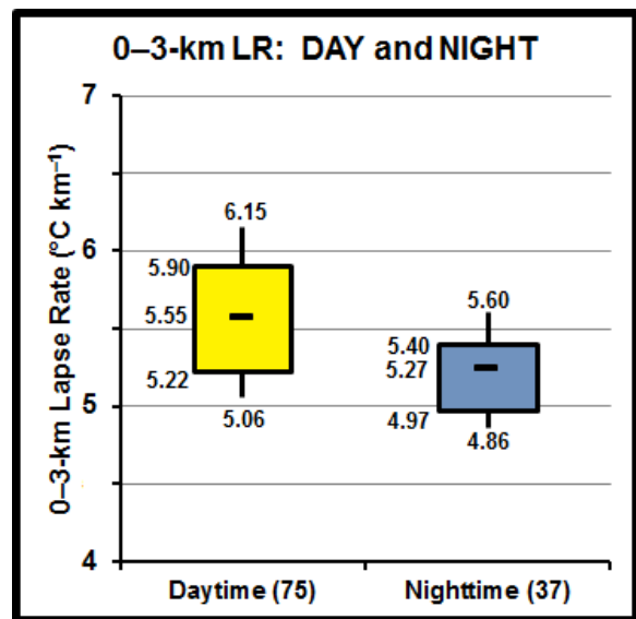
Figure 6: Boxplots of 0–3-km AGL lapse rate ( \text{C km}^{-1} ) by day (yellow) and night (slate blue), as defined in the text. Box and whisker percentiles same as in preceding figures.
