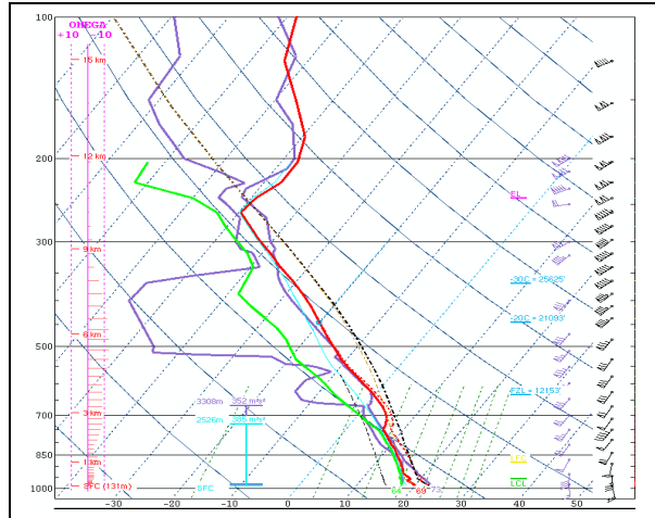
Fig 5. Eta-kt 21 hr forecast valid at 00z Feb. 6 th overlaid with observed sounding valid the same time. Red- temperature and green- dew point for the forecast Eta-kt sounding. Obs. in purple.
