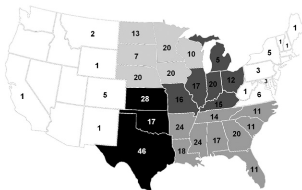
FIG. 3. Numbers of significant tornado events by state. Geographic regions are noted by filled groupings (northern Great Plains in light gray, southern Great Plains in black, Midwest in dark gray, and Southeast in medium gray).
