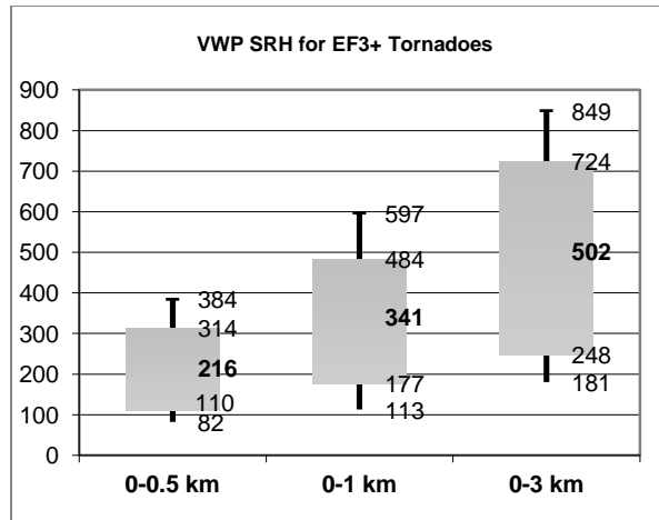
Figure 4. Same as Fig. 3, except 0-0.5 km SRH, 0-1 km SRH, and 0-3 km SRH ( \text{m}^2/\text{s}^2 ).
