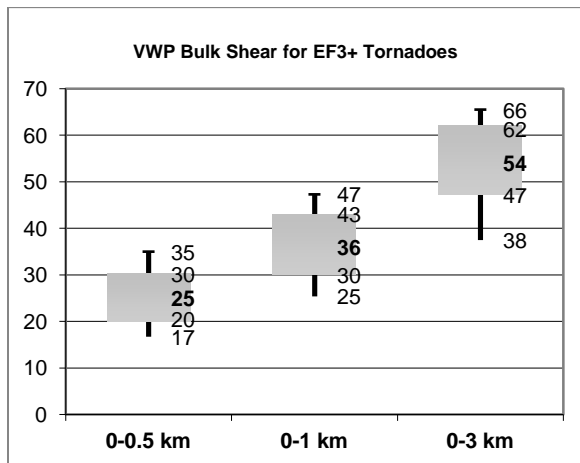
Figure 3. Box and whisker diagrams of low-level (0-0.5, 0-1, & 0-3 km AGL) bulk shear (kt) for EF3+ tornadoes \leq 75 km of WSR-88D VWP for 2008-2011. Each box is representative of the 25 th to 75 th percentiles of values with the mean value in the middle. The outer whiskers represent the 10 th and 90 th percentiles.
