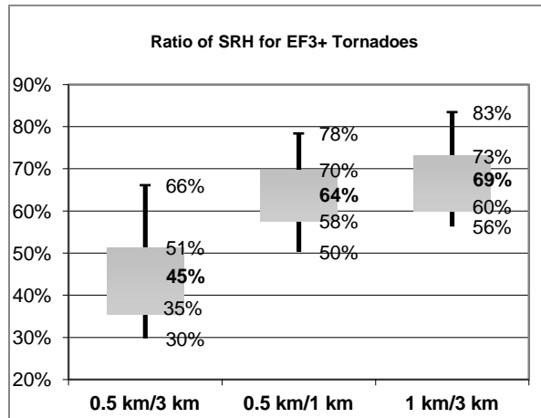
Figure 5. Same as Fig. 3, except ratio of 0-0.5 km SRH to 0-3 km SRH, 0-0.5 km SRH to 0-1 km SRH, and 0-1 km SRH to 0-3 km SRH ( \text{m}^2/\text{s}^2 ).
