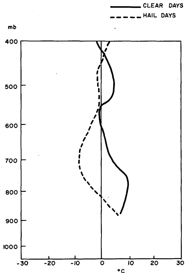
FIG. 8. Profile of average temperature departure from mean conditions for five clear and five hail days at Sterling, Colo. (after Modahl, 1974).
