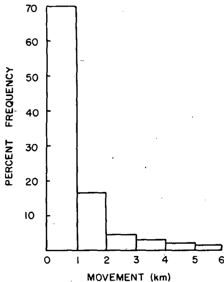
FIG. 3. Frequency distribution of total echo movement over Arizona during 1955.
