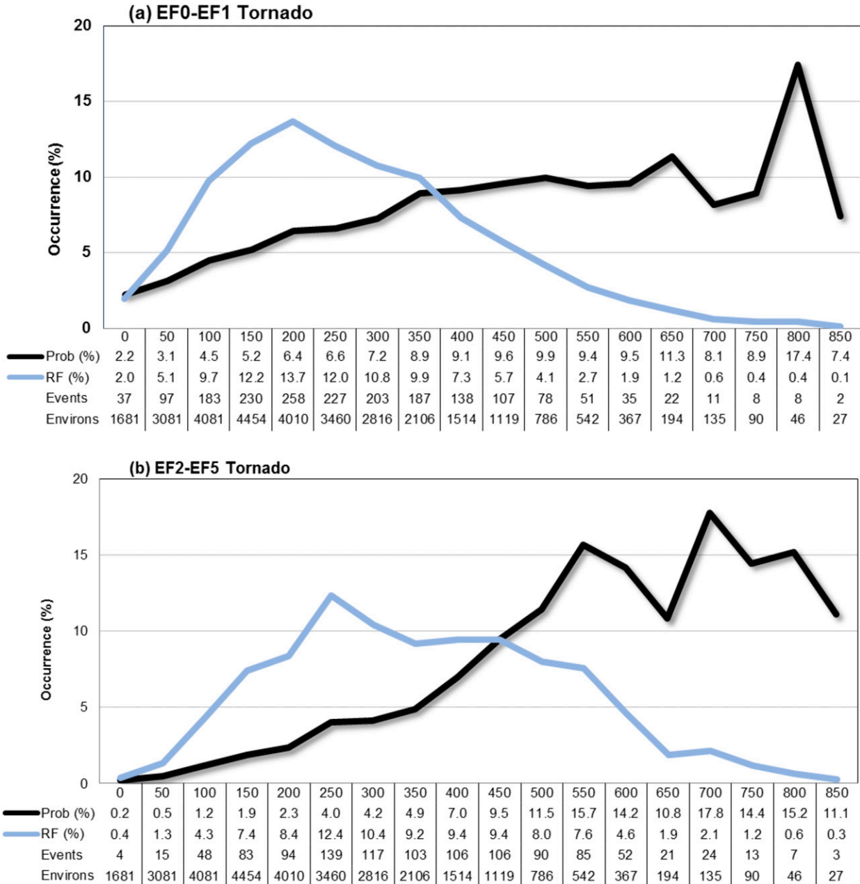
FIG. 10. The Prob (black) and RF (blue) plots for effective SRH ( \text{m}^2 \text{s}^{-2} ) corresponding to (a) weak and (b) significant tornado events. These plots use constraints for organized, surface-based convection: effective bulk shear at least 50 kt, MLCAPE at least 1000 \text{ J kg}^{-1} , MLCIN less negative than or equal to -50 \text{ J kg}^{-1} , and MLLCL at or below 1500 m.
