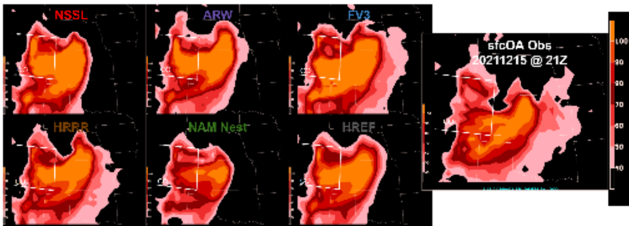
Figure 10. Forecasts of the FFWI for the NSSL (top left), ARW (top middle), FV3 (top right), HRRR (bottom left), NAM Nest (bottom middle), and HREF (bottom right) with the analysis (far right) valid at 2100 UTC on 15 December 2021 for the historic wildfire event across portions of the Central and Southern Plains.
