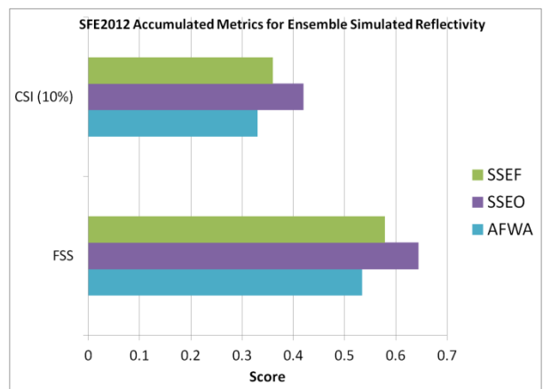
Figure 3. The accumulated CSI (10%) and FSS for each ensemble during the SFE2012 for smoothed neighborhood probabilities of simulated reflectivity \geq 40 dBZ.
