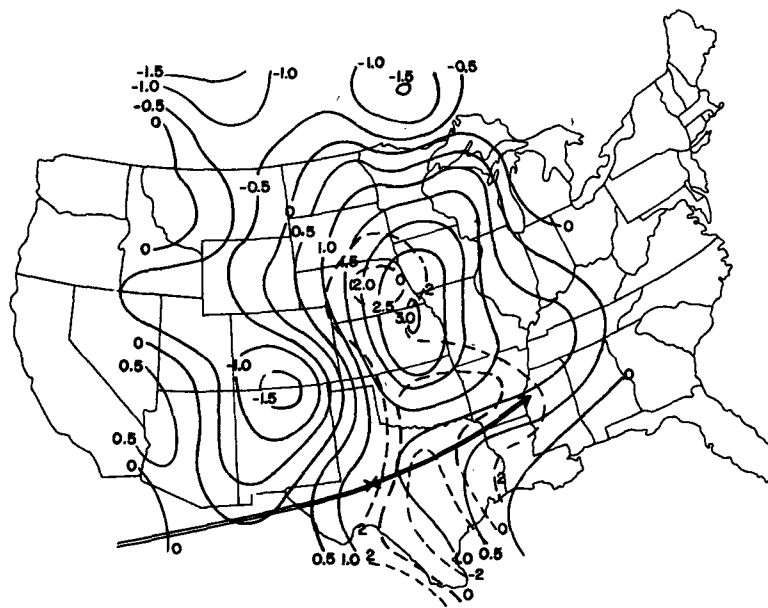
FIG. 10a. Mean divergence in 200-300 mb layer (solid, 10^{-6} \text{ s}^{-1} ) and SELS lifted index (dashed, ^{\circ}\text{C} ); arrow is 300 mb axis of maximum wind; X is wind maximum center; 0000 GMT 3 March 1977.
