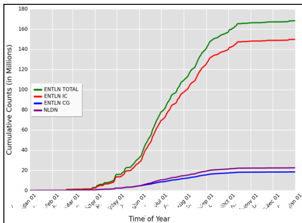
Figure 1: Running annual tally of hourly lightning flashes in 2014 from QC-CG NLDN. For comparison, total lightning counts from ENTTLN as well as the corresponding CG and IC flash components are provided.
