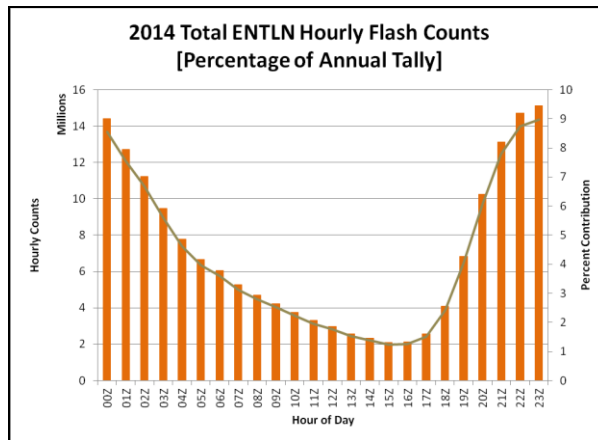
Figure 2: 2014 Total ENTTLN hourly flash counts (in millions) and percentages of annual tally.
