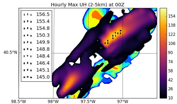
Figure 12 As Figure 2, but for the hour ending at 00UTC on 12 May 2014.
