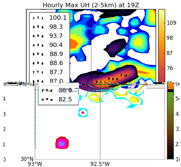
Figure 5 As Figure 2, but for 19UTC
