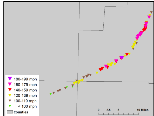
Figure 5. Similar to Fig. 1 except for estimated wind speeds associated with the DIs.
