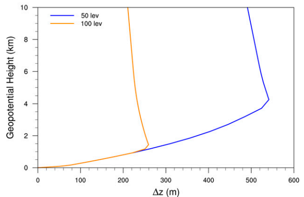
FIG. 2. A line graph depicting the vertical grid spacing ( \Delta z ; m) between WRF eta vertical levels, delineated by corresponding domain-averaged geopotential heights for runs employing 50 vertical levels (blue line) and 100 vertical levels (orange line). Geopotential heights were only plotted up to 10 km to adequately show how \Delta z in runs employing 50 and 100 vertical levels varies with height and does not extend to the model top.
