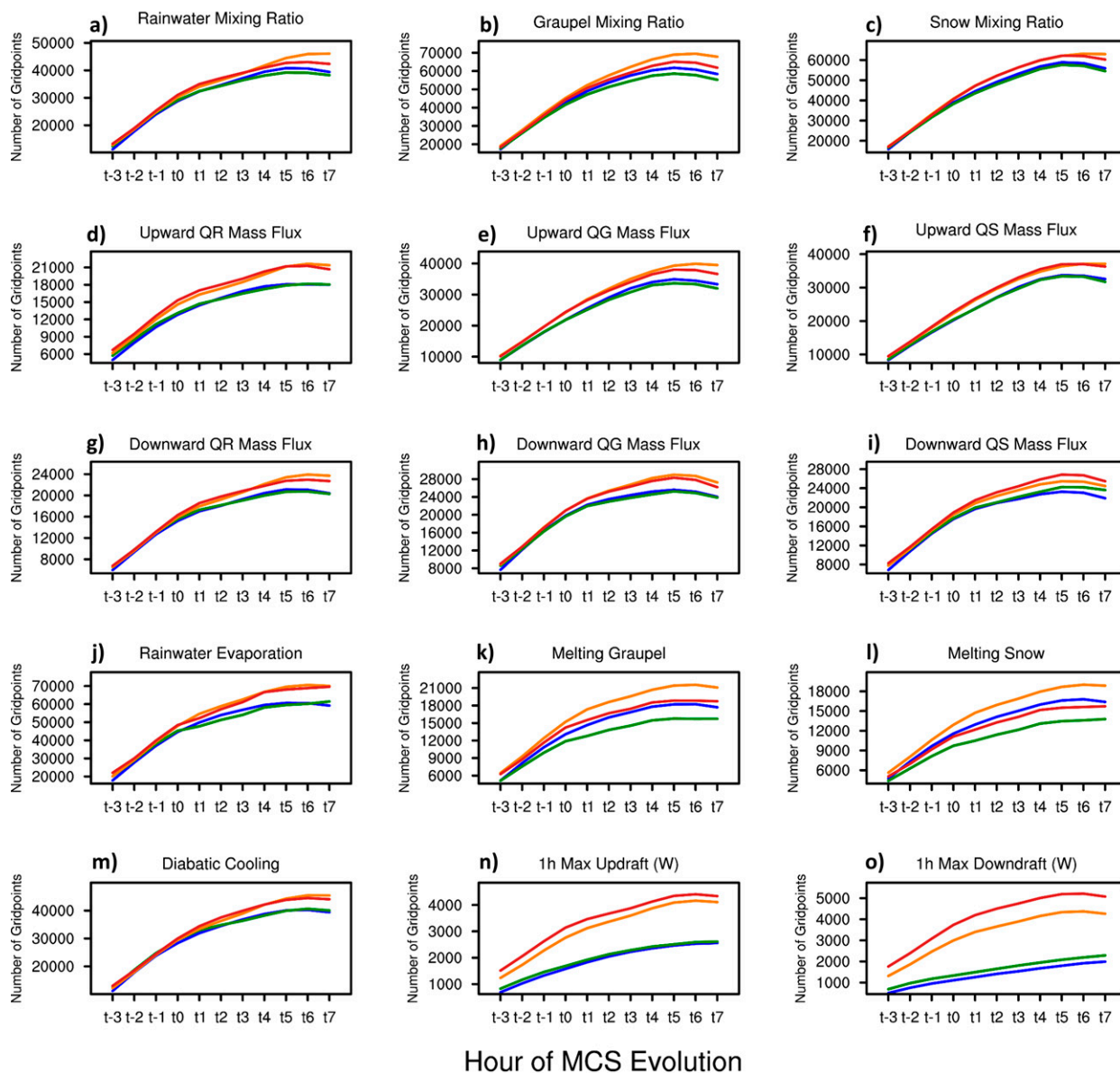
FIG. 18. As in Fig. 14, but for WSM6 MP simulations.
