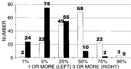
FIG. 2. Forecasts of (left) one or more tornadoes and (right) three or more tornadoes by probability.
